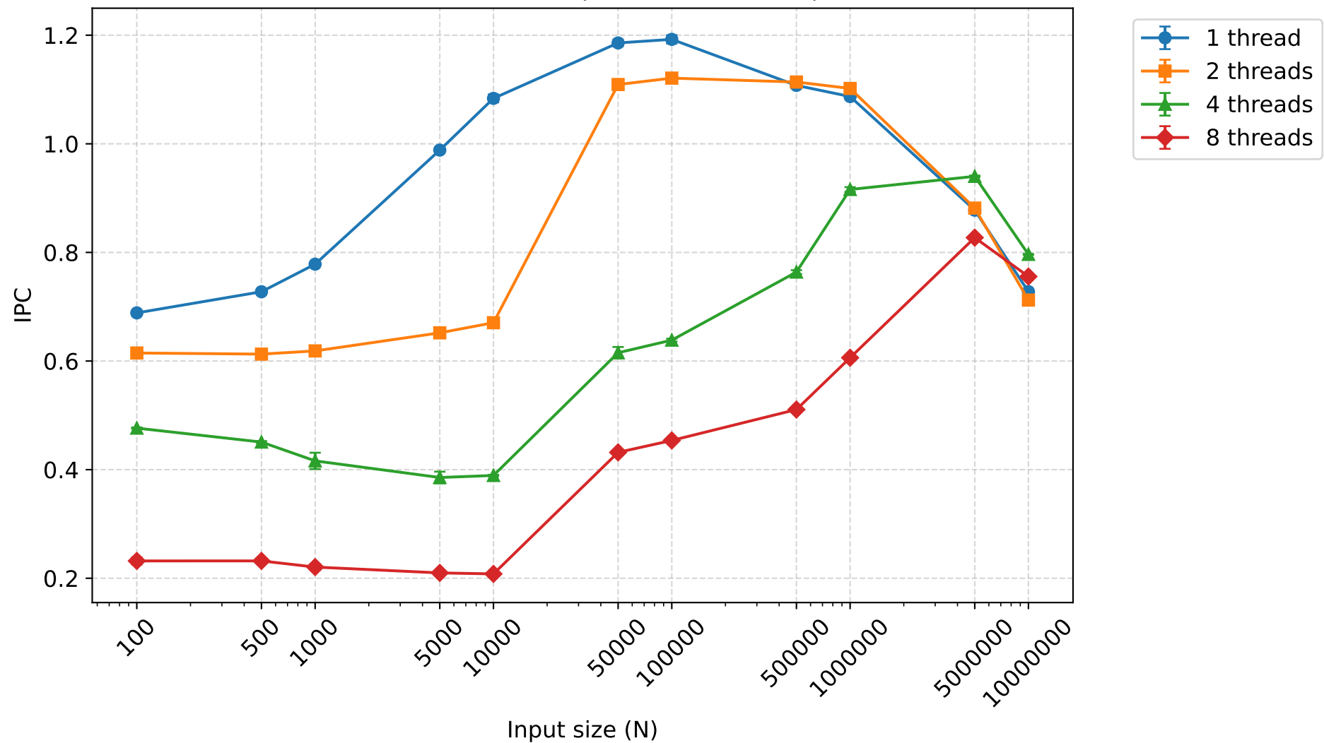
IPC - smoothsort (mean \pm 95% CI)
