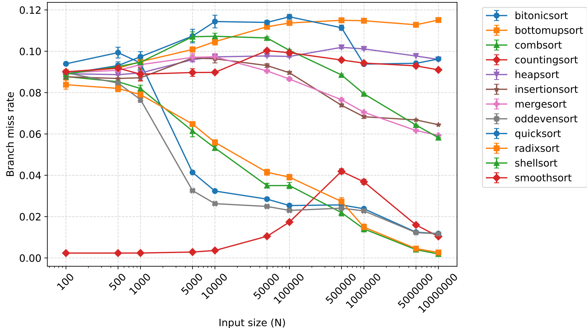
Branch miss rate - 4 threads (mean \pm 95% CI)
