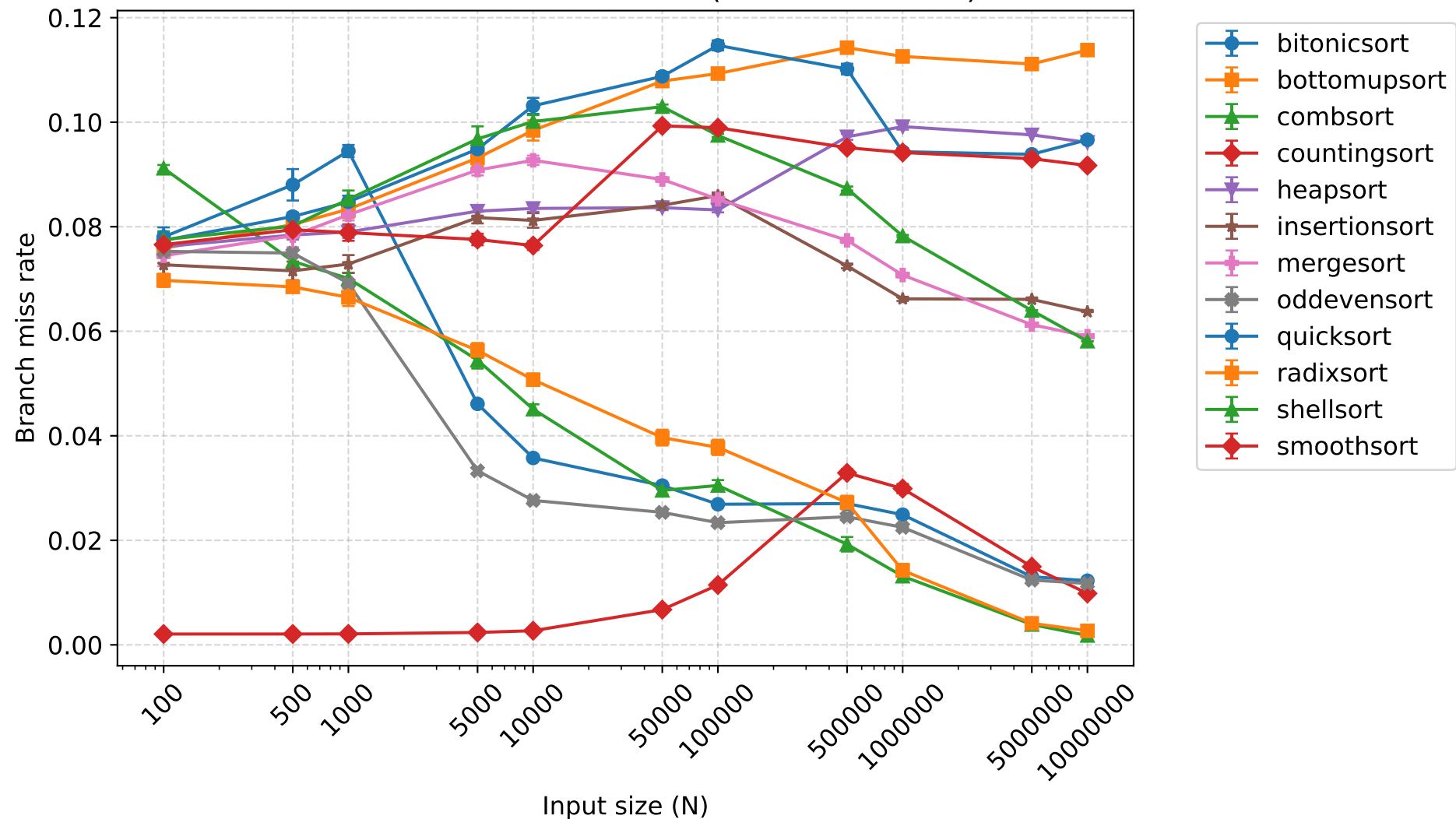
Branch miss rate - 8 threads (mean \pm 95% CI)
