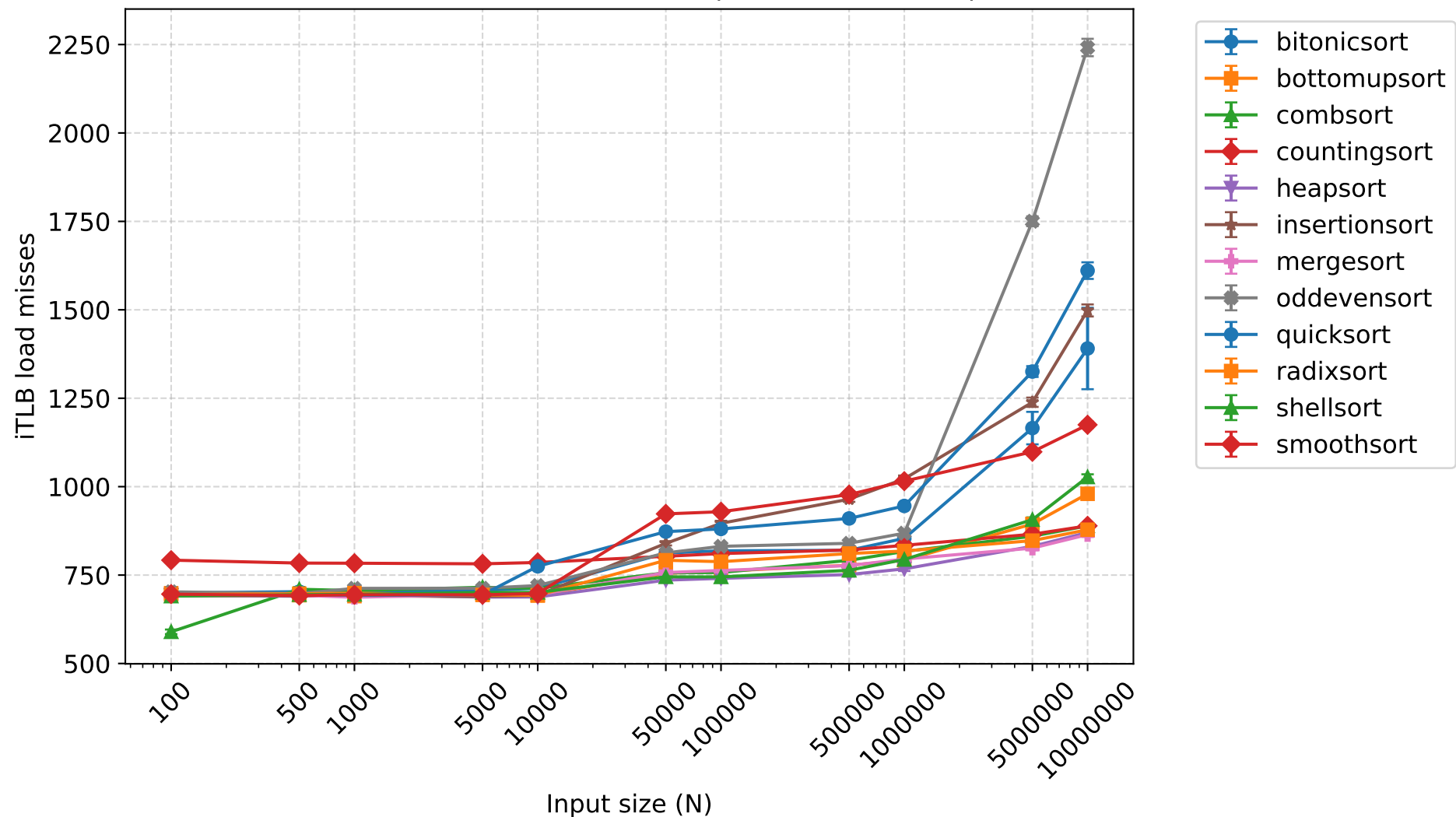
iTLB load misses - 8 threads (mean \pm 95% CI)
