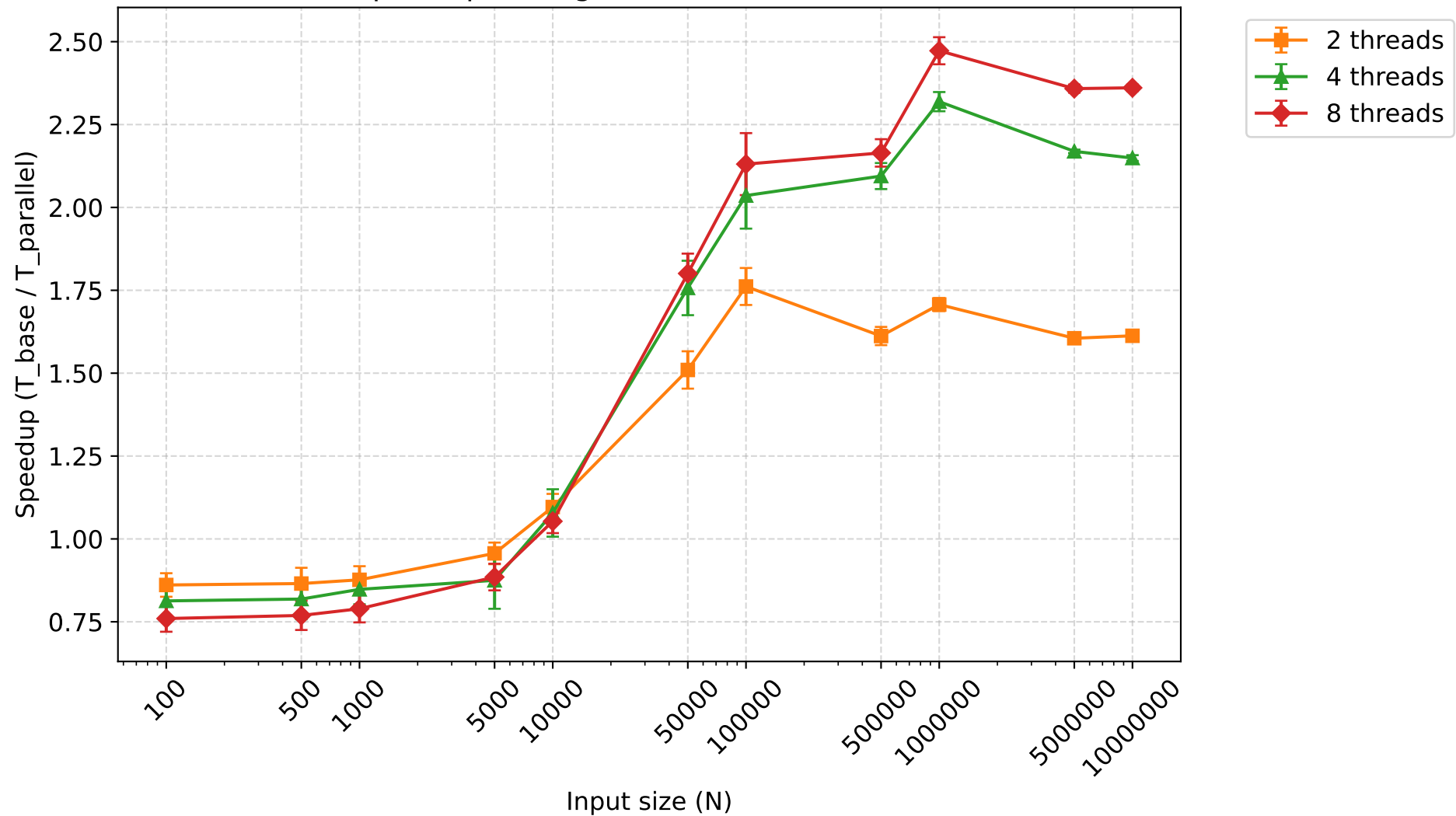
Speedup - mergesort (mean \pm 95% CI)
