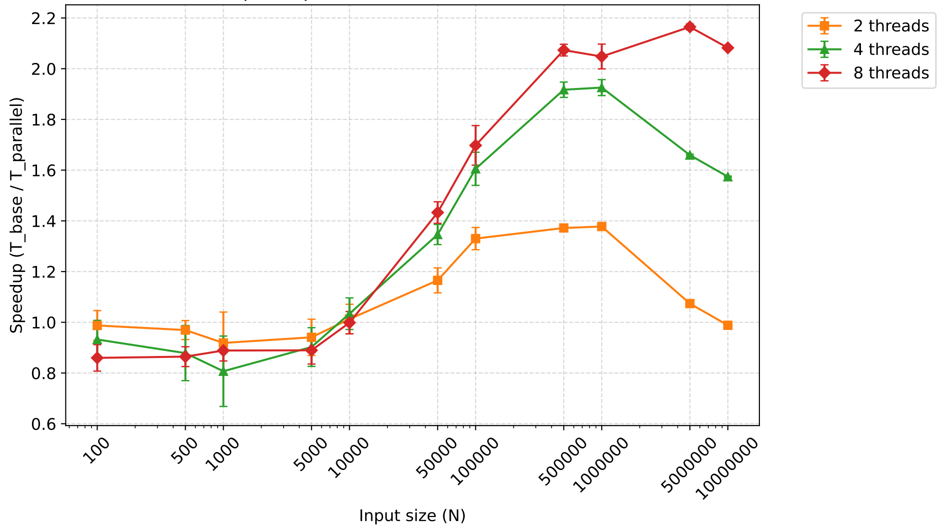
Speedup - shellsort (mean +- 95% CI)
