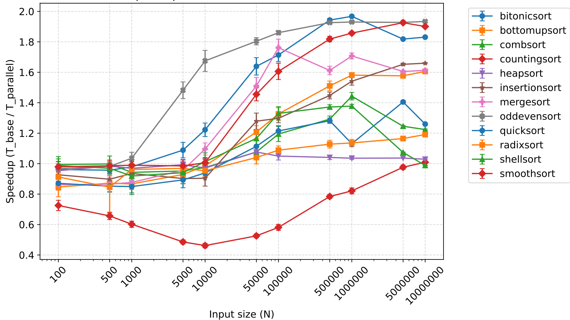
Speedup - 2 threads (mean +- 95% CI)
