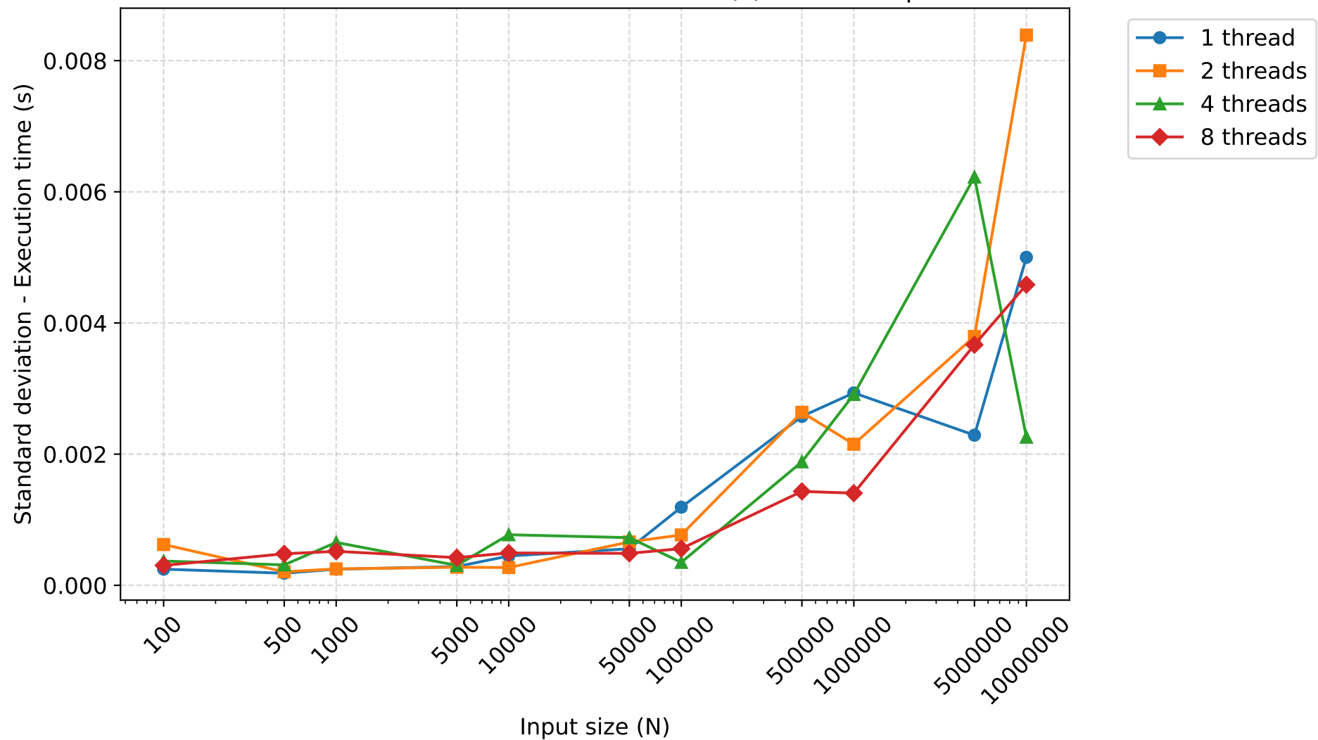
Standard deviation of Execution time (s) - bottomupsort
