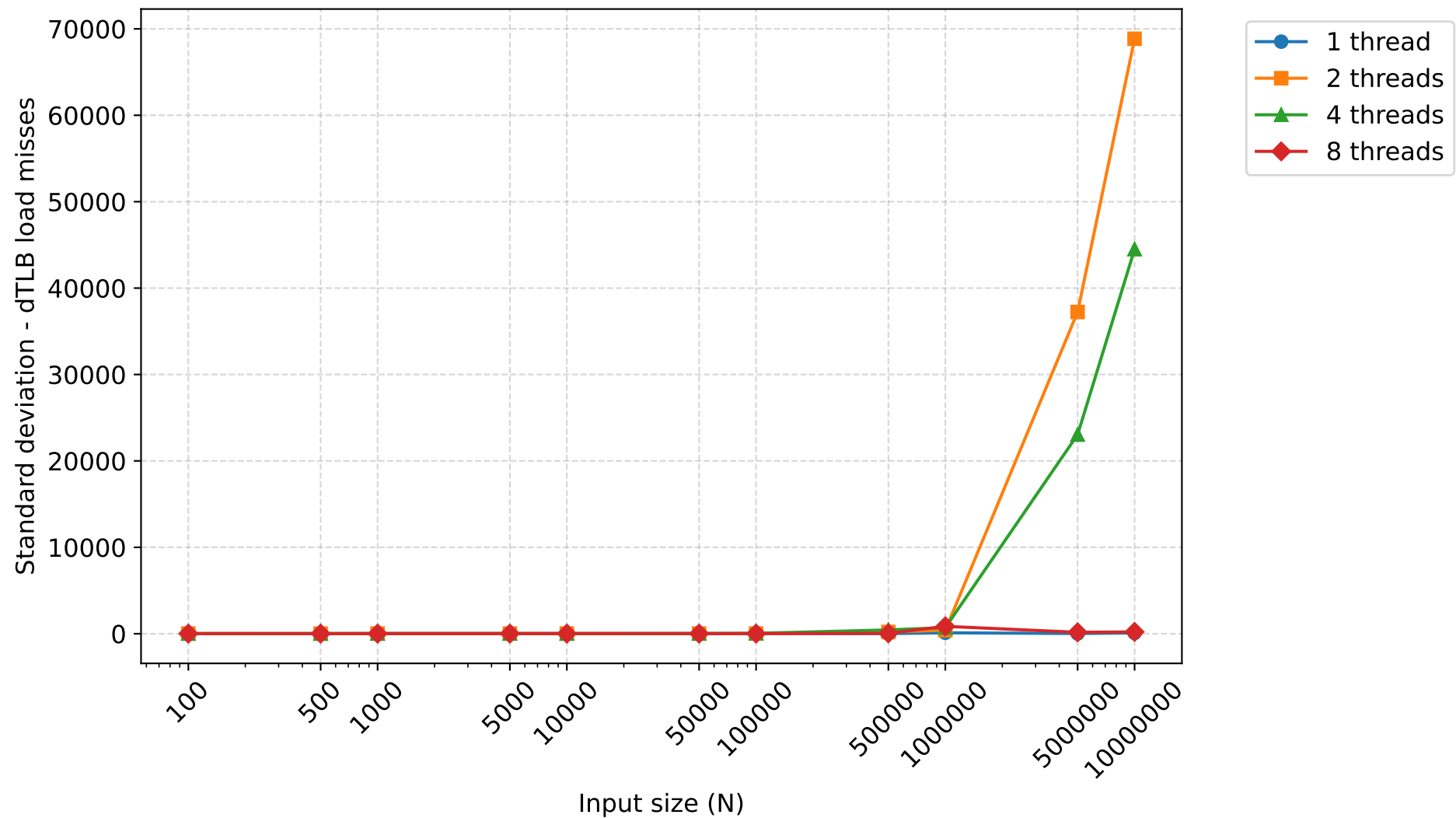
Standard deviation of dTLB load misses - combort
