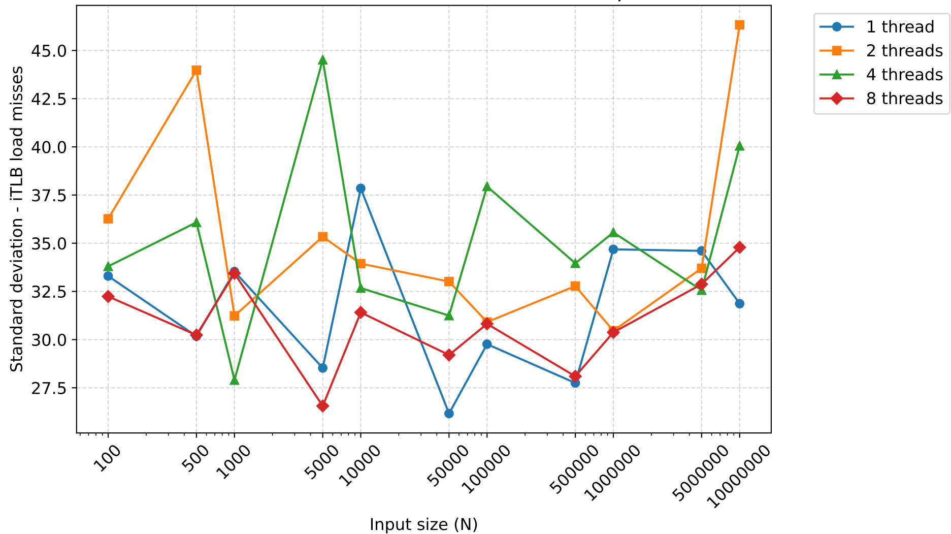
Standard deviation of iTLB load misses - heapsort
