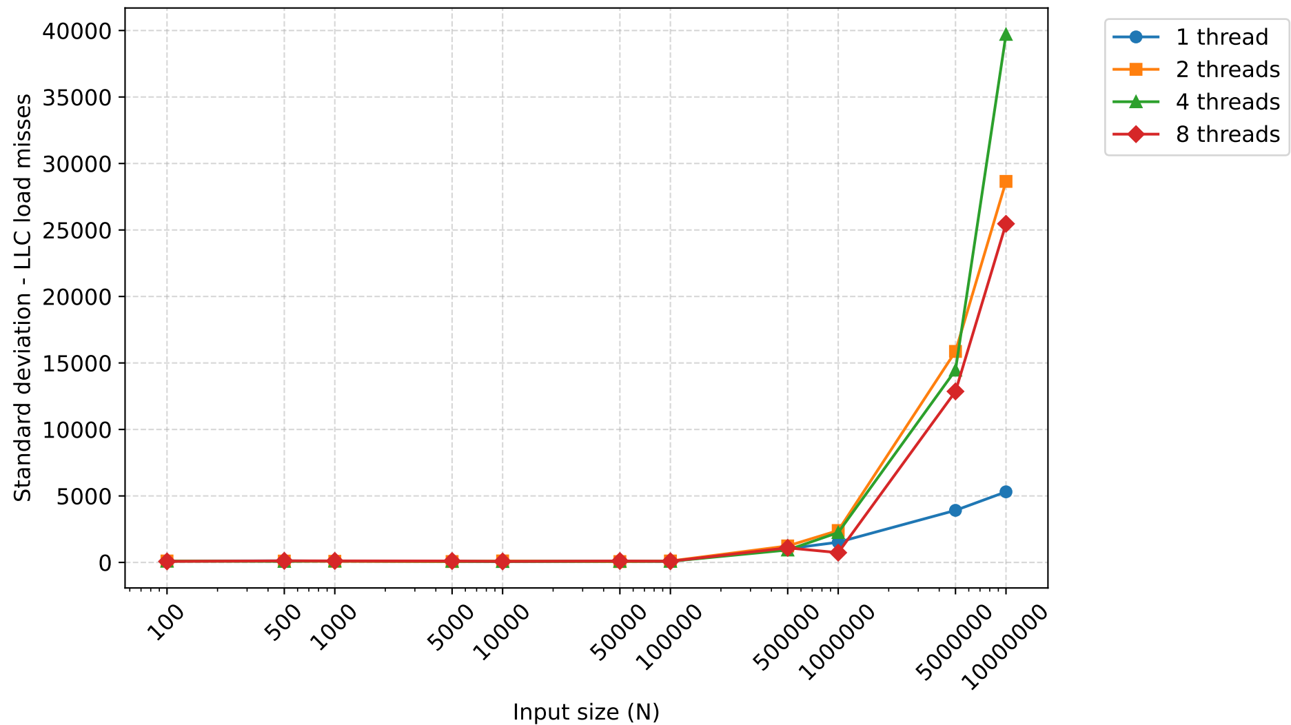
Standard deviation of LLC load misses - insertionsort
