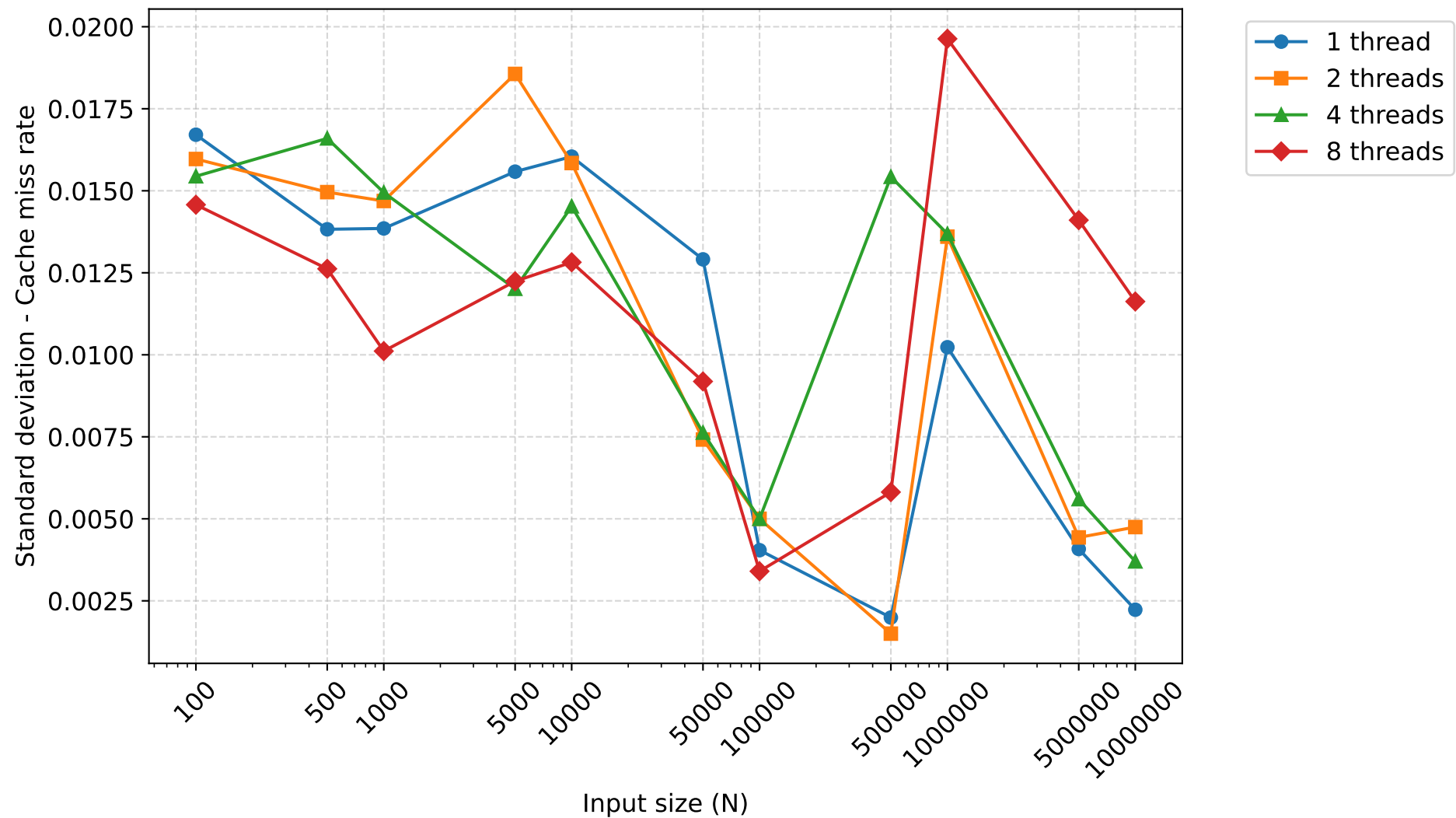
Standard deviation of Cache miss rate - insertionsort
