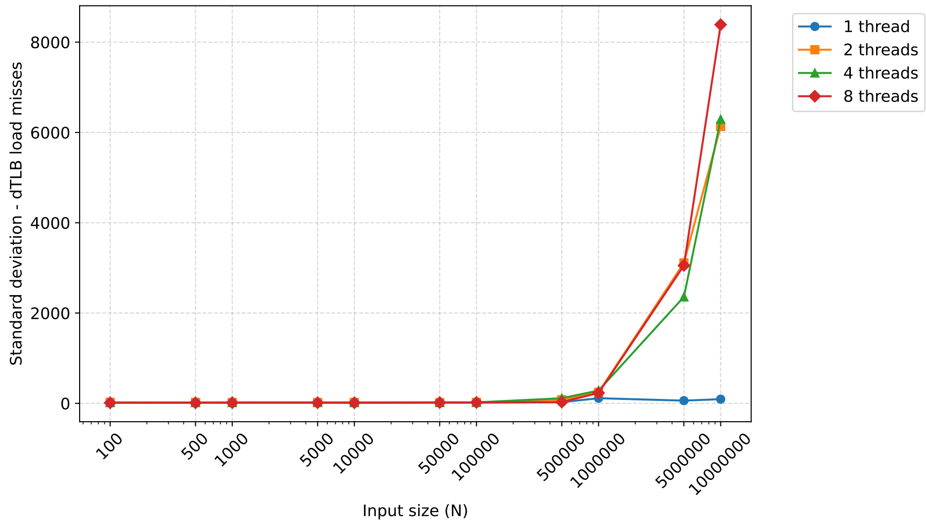
Standard deviation of dTLB load misses - insertionsort
