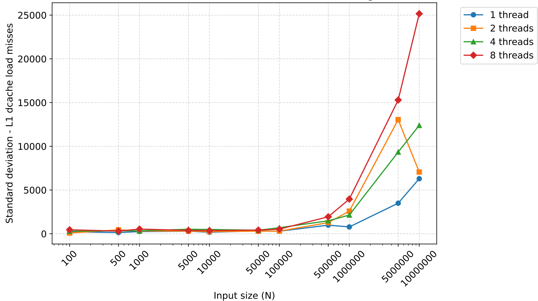
Standard deviation of L1 dcache load misses - mergesort
