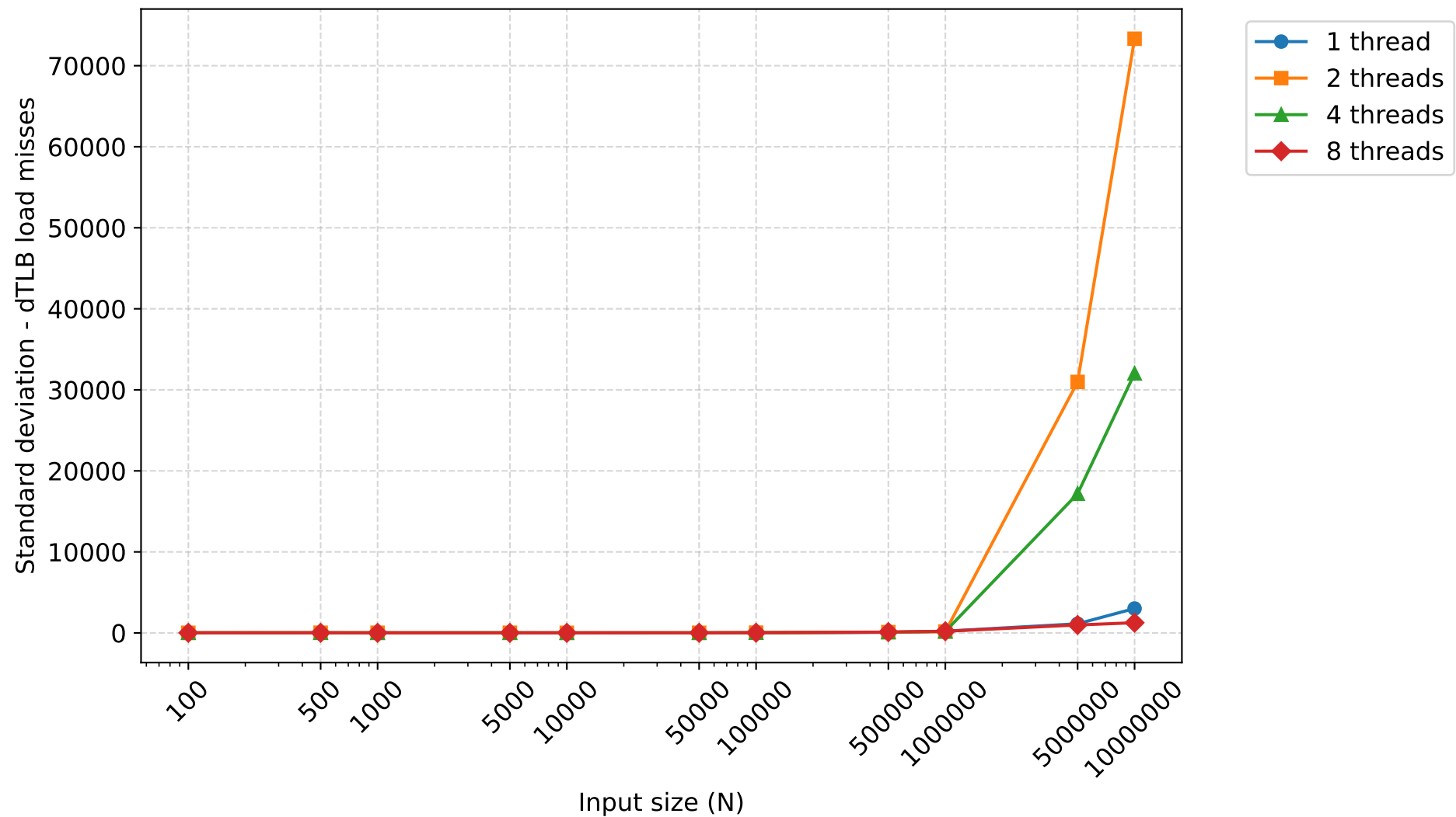
Standard deviation of dTLB load misses - oddeven sort
