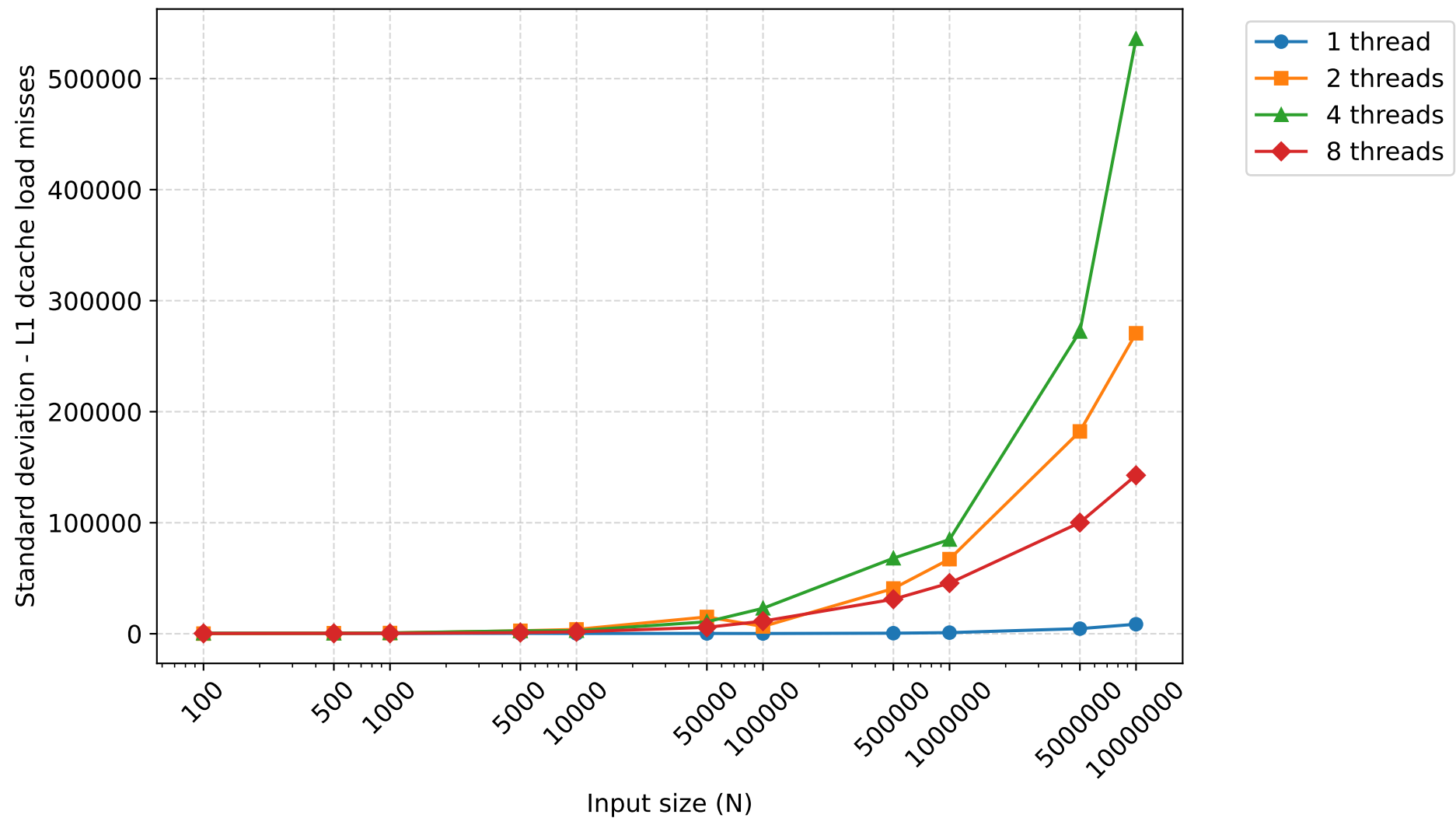
Standard deviation of L1 dcache load misses - radixsort
