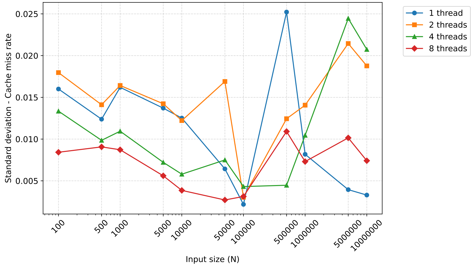
Standard deviation of Cache miss rate - radixsort
