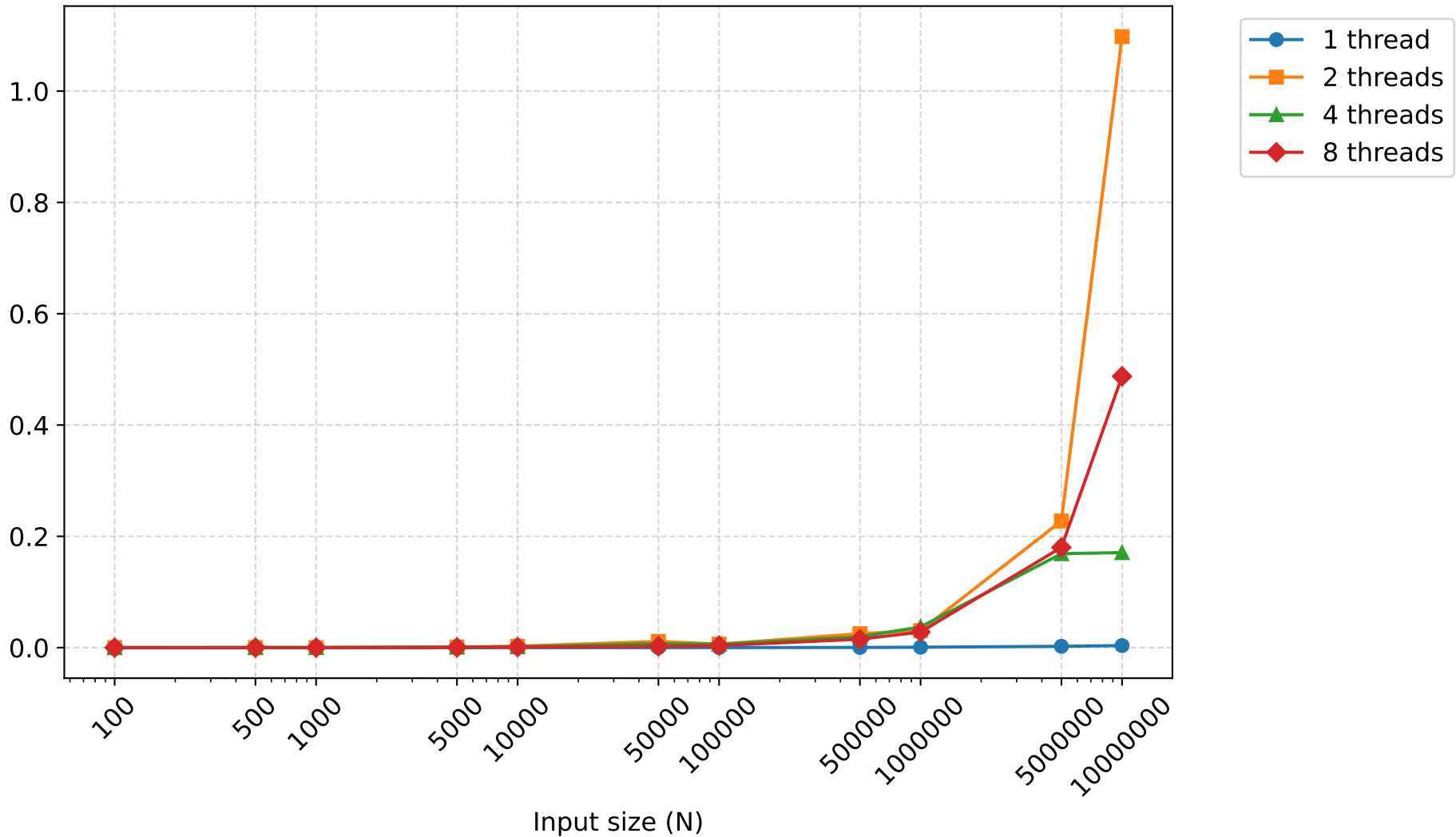
Standard deviation of L1 dcache load misses - shellsort
