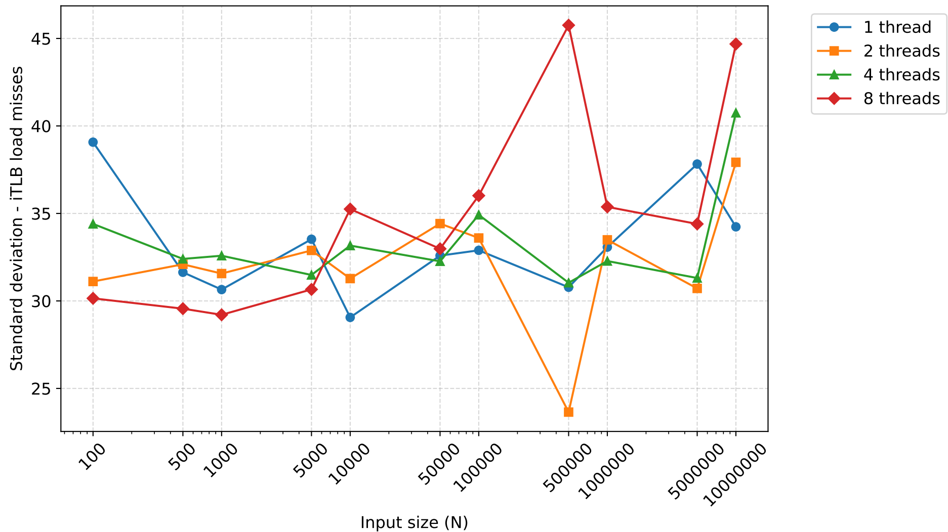
Standard deviation of iTLB load misses - smoothsort
