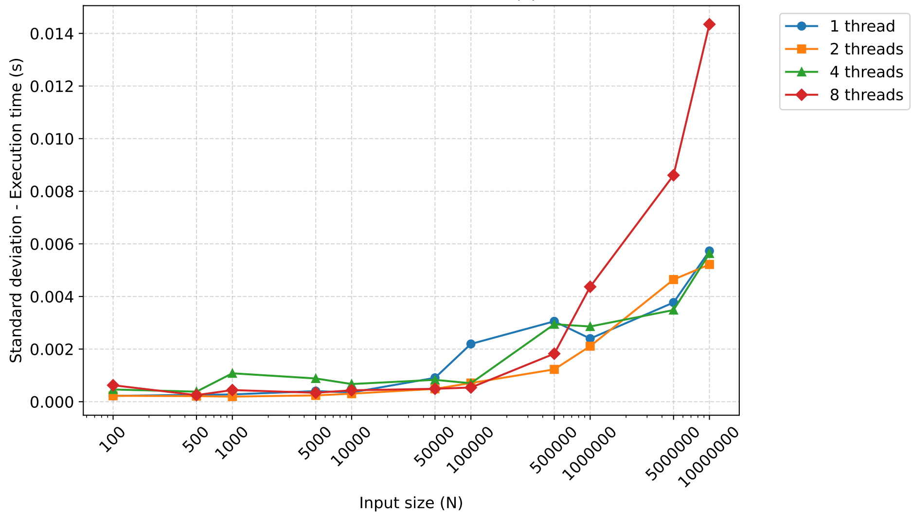
Standard deviation of Execution time (s) - smoothsort
