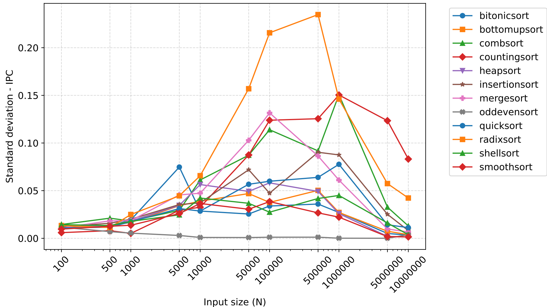
Standard deviation of IPC - 1 thread
