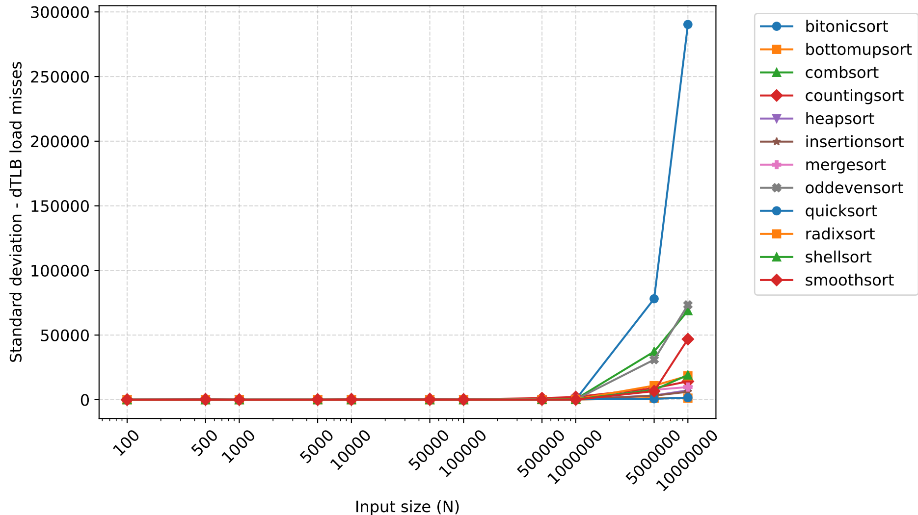
Standard deviation of dTLB load misses - 2 threads
