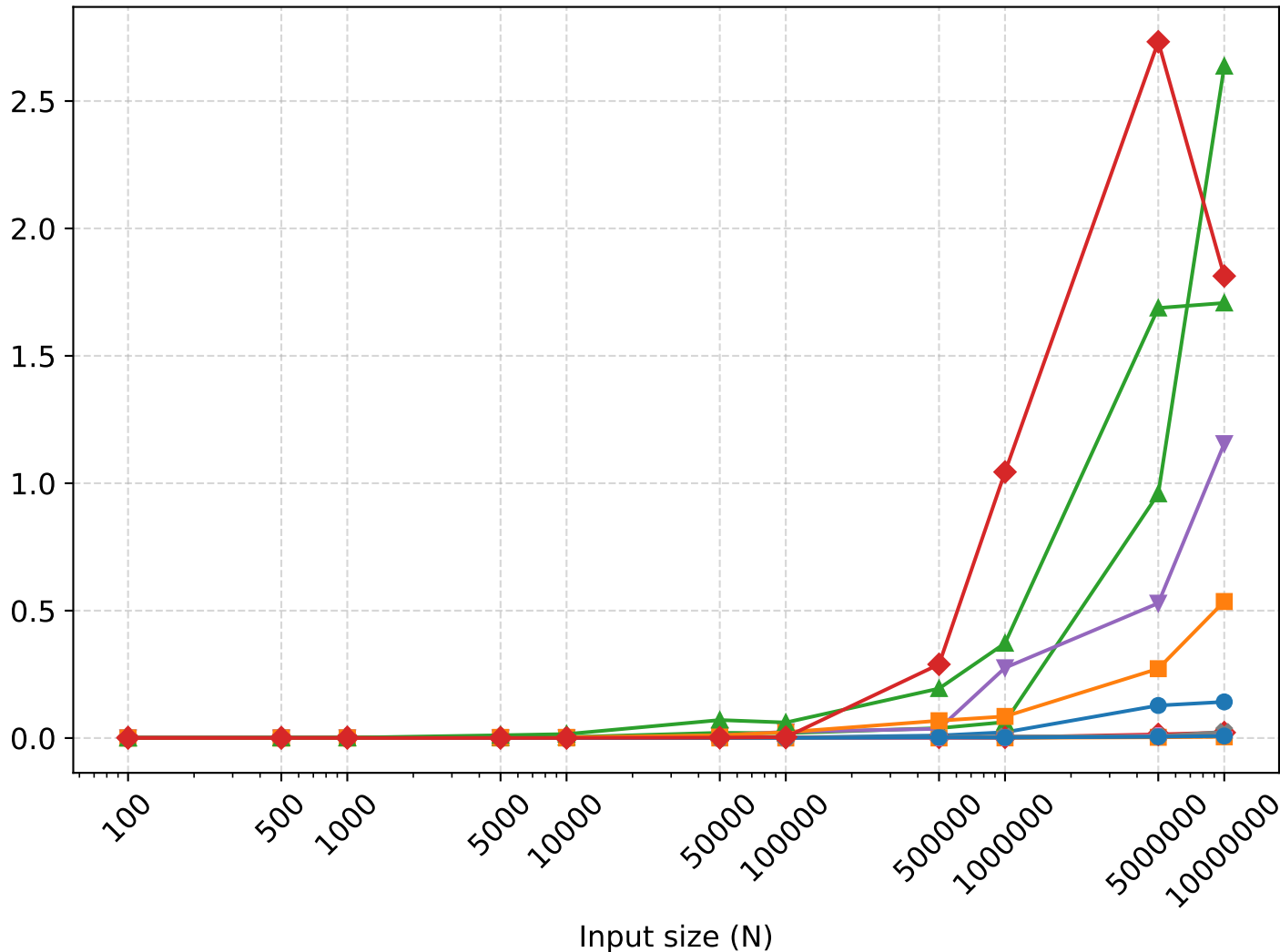
Standard deviation of L1 dcache load misses - 4 threads
