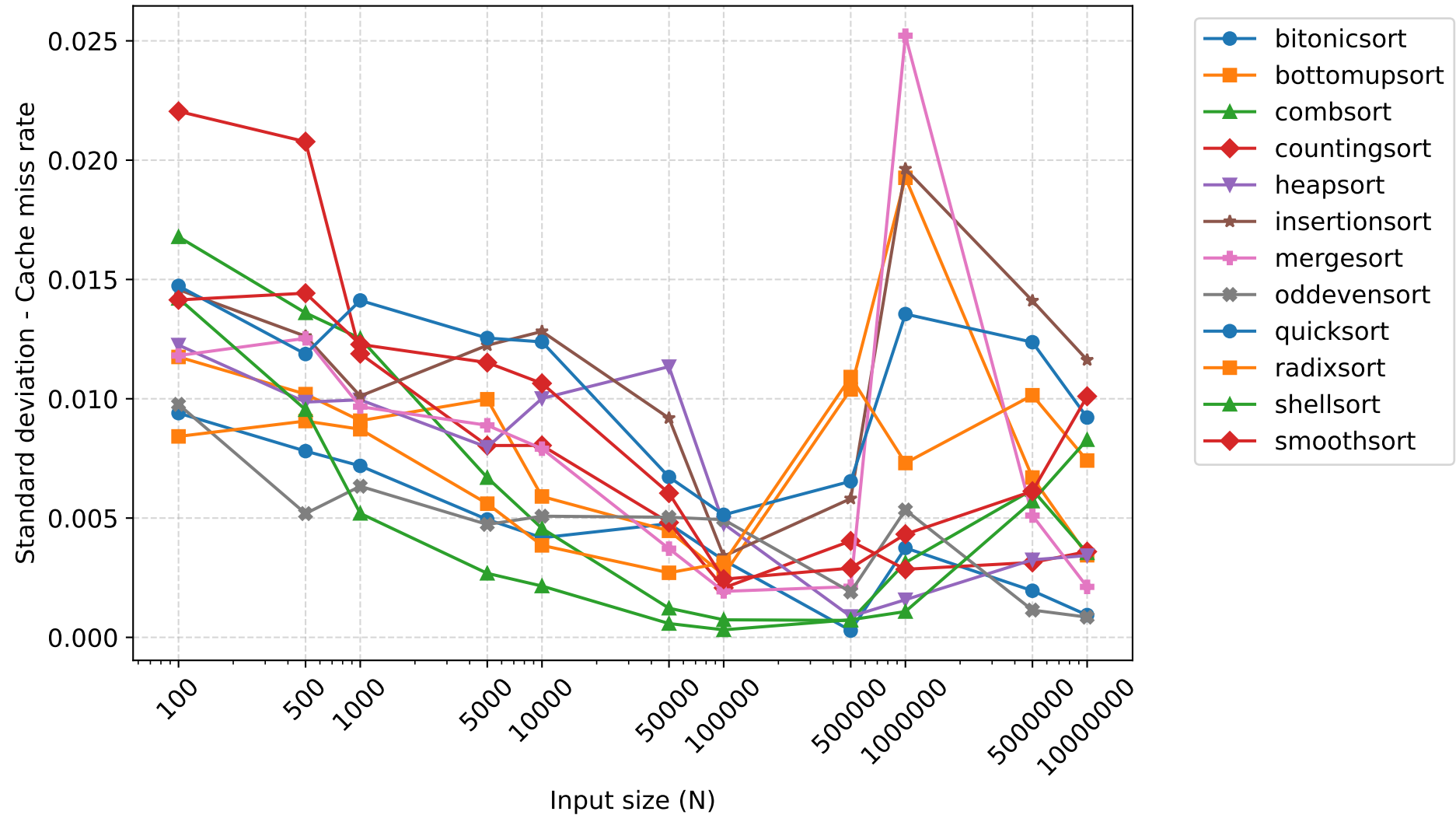
Standard deviation of Cache miss rate - 8 threads
