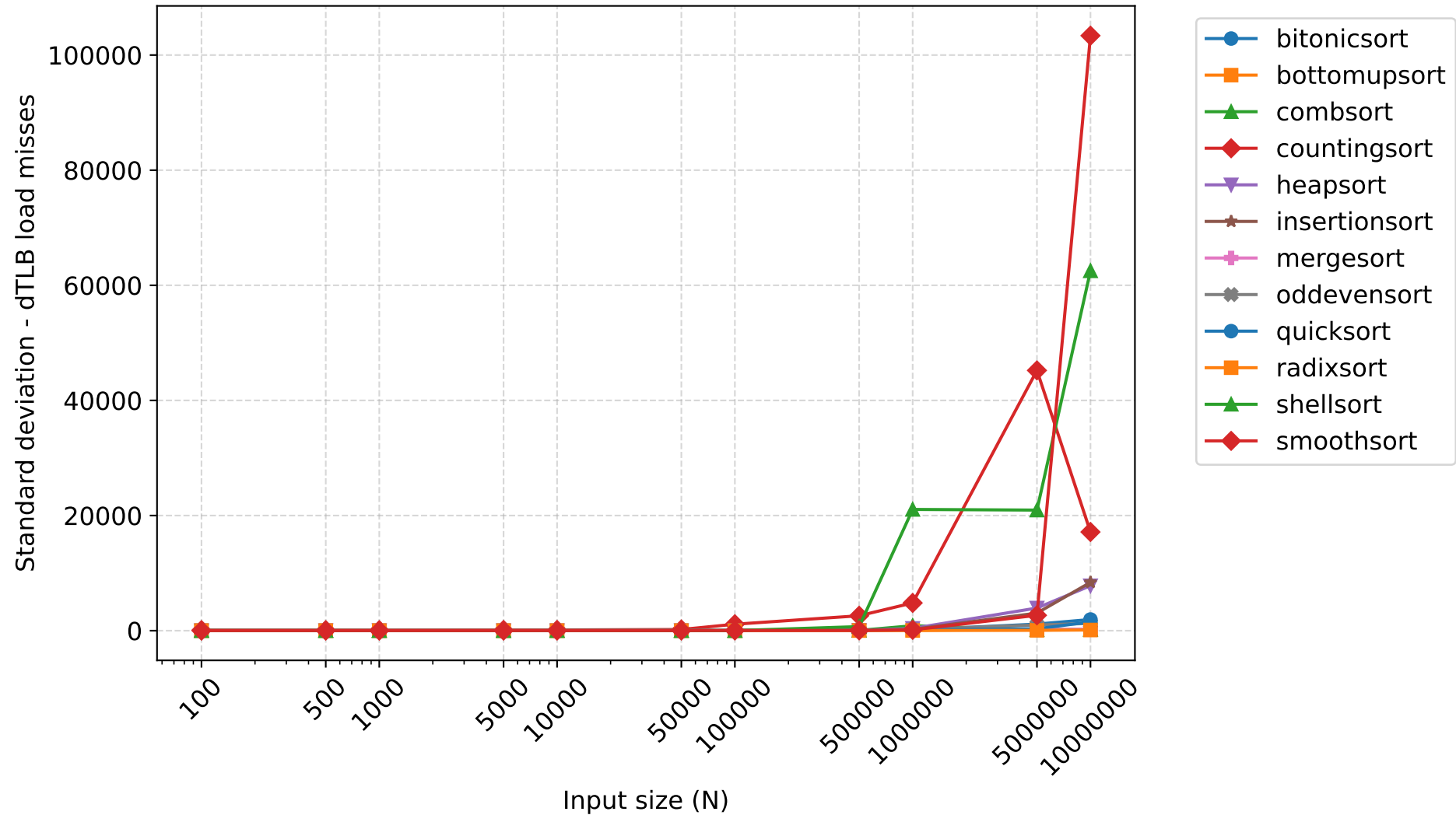
Standard deviation of dTLB load misses - 8 threads
