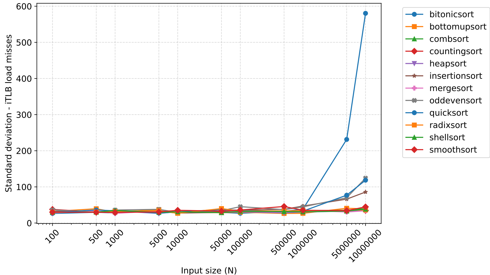
Standard deviation of iTLB load misses - 8 threads
