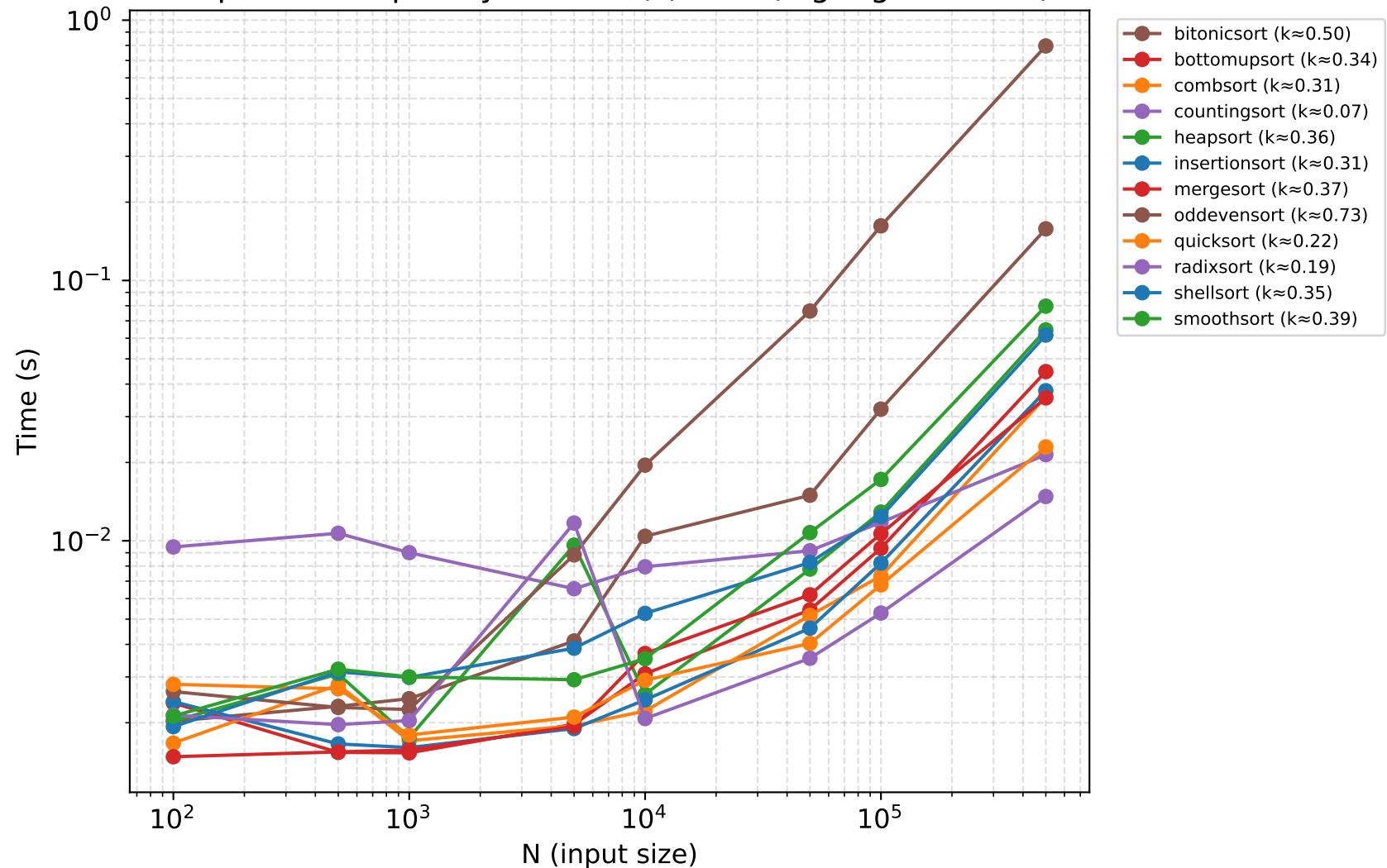
Empirical complexity — Time (s) vs N (log-log, serial t1)
