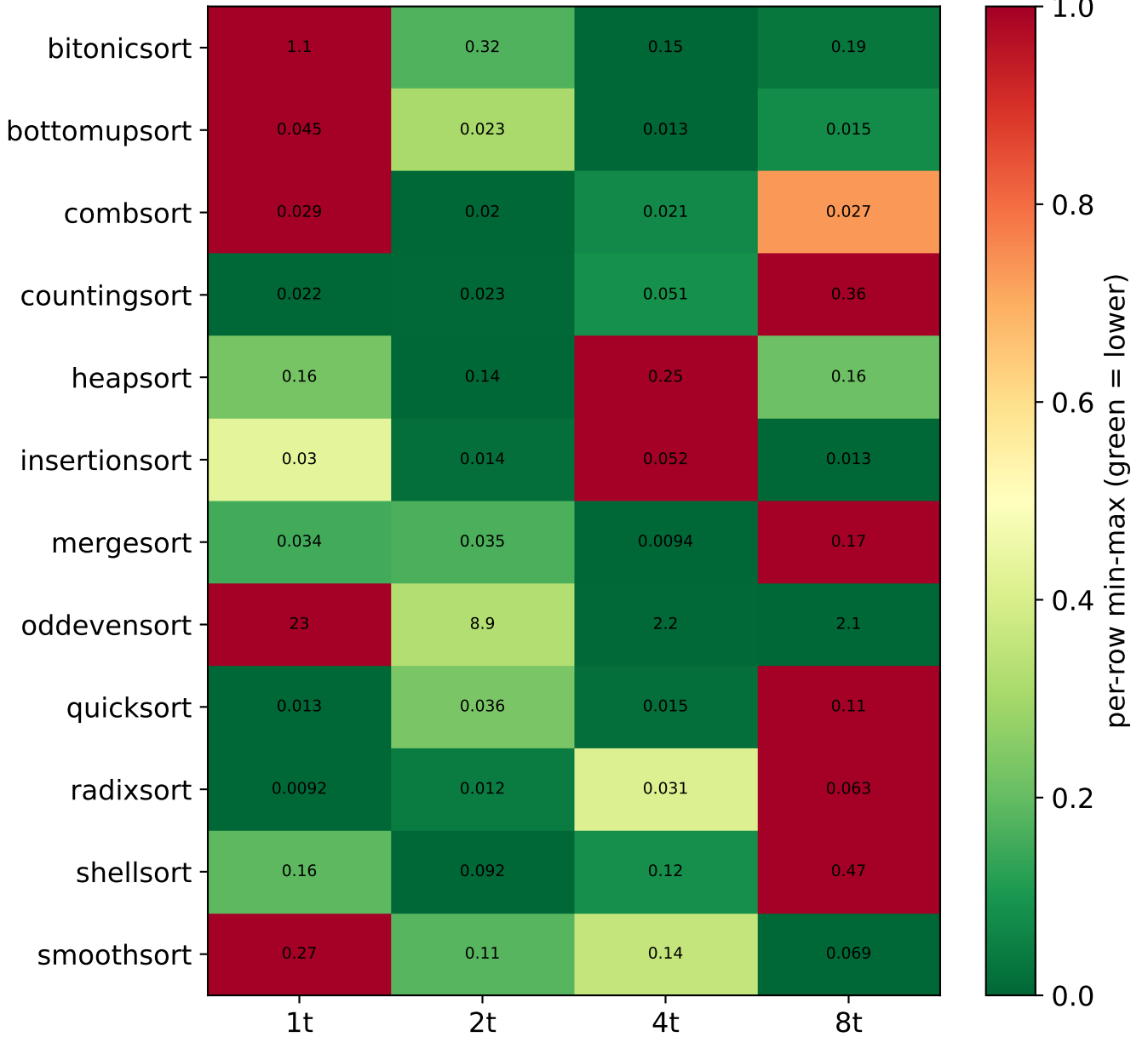
EDP (J·s) by algorithm x threads ( N = 500000 ) — green = best per row
