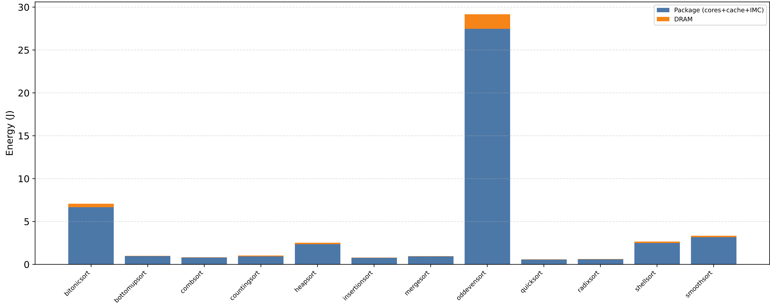
Energy breakdown: package vs DRAM ( N = 500000 , serial)
