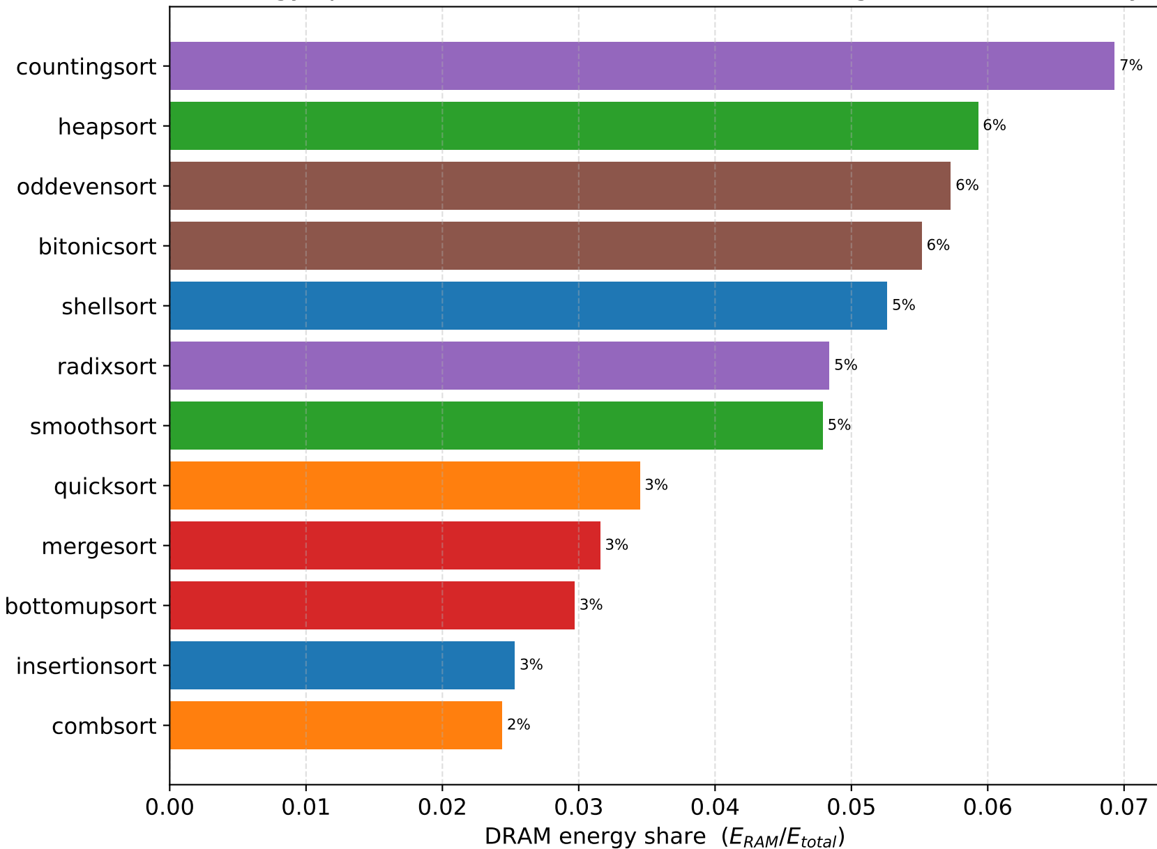
Share of energy spent in DRAM ( N = 500000 , serial) — higher = more memory-bound
