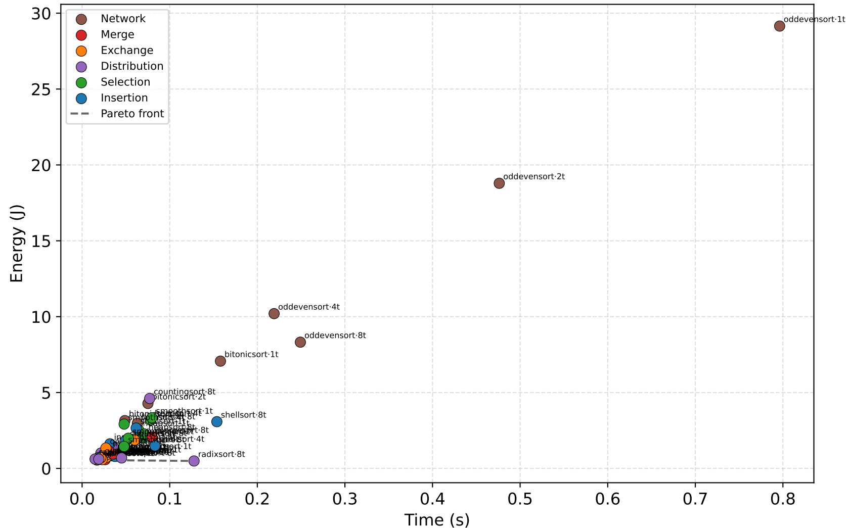
Energy-time trade-off ( N = 500000 , all thread counts)
