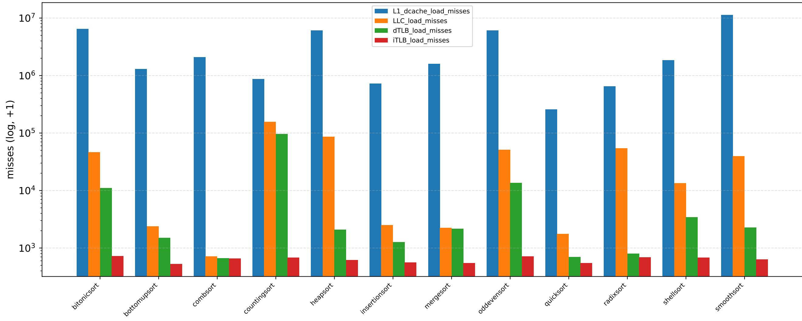
Memory hierarchy pressure ( N = 500000 , serial)
