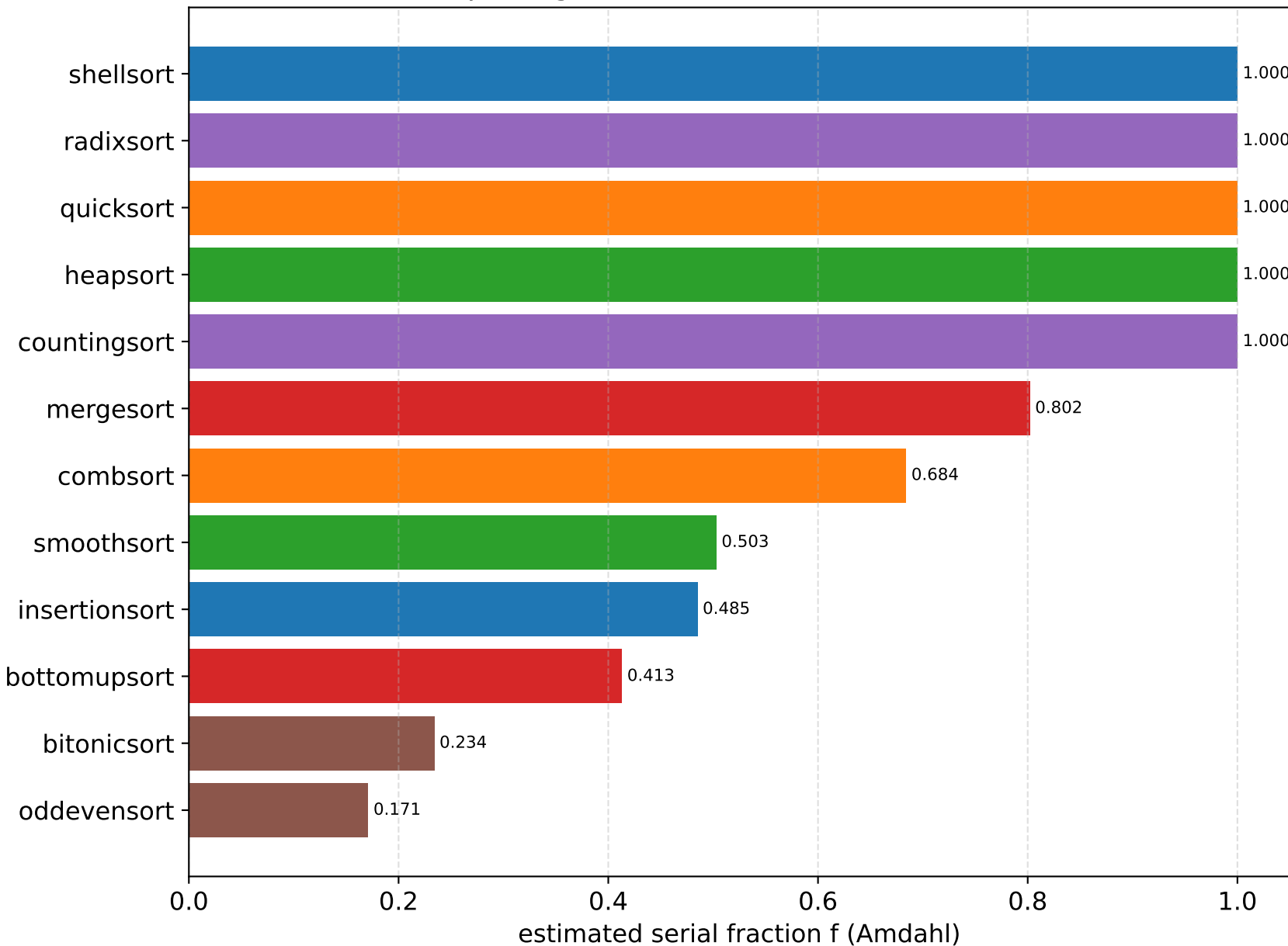
Serial fraction per algorithm ( N = 500000 ) — lower f scales better
