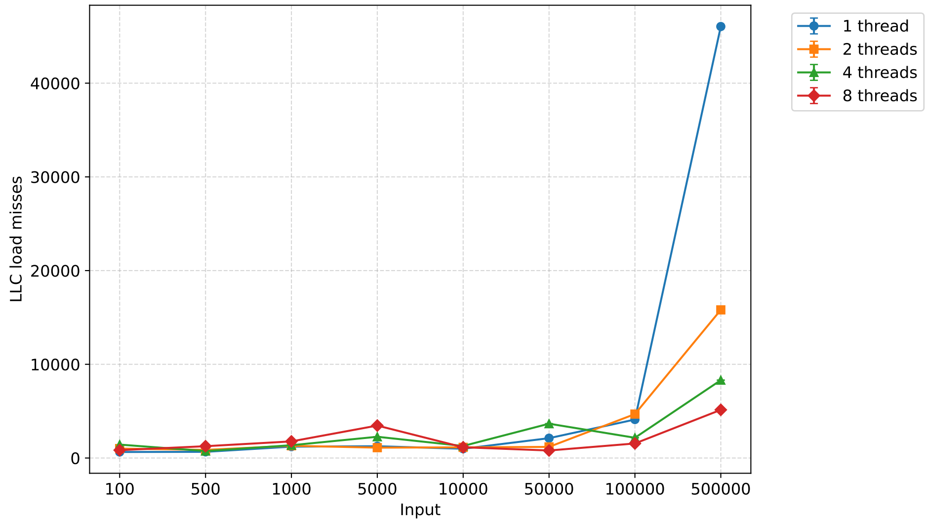
LLC load misses - bitonicsort (mean \pm 95% CI)
