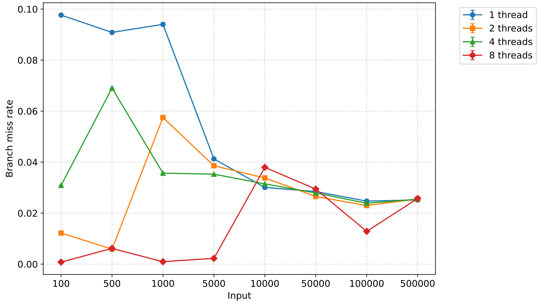
Branch miss rate - bitonicsort (mean \pm 95% CI)
