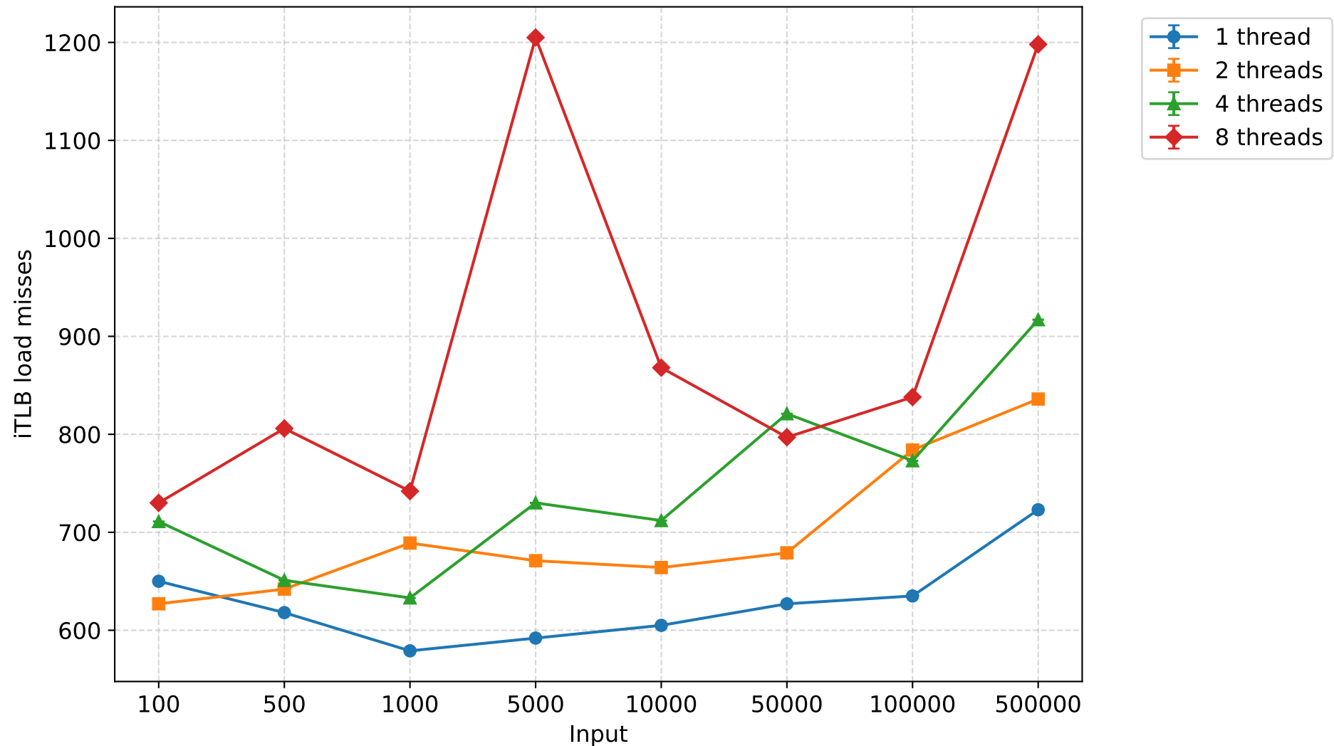
iTLB load misses - bitonicsort (mean \pm 95% CI)
