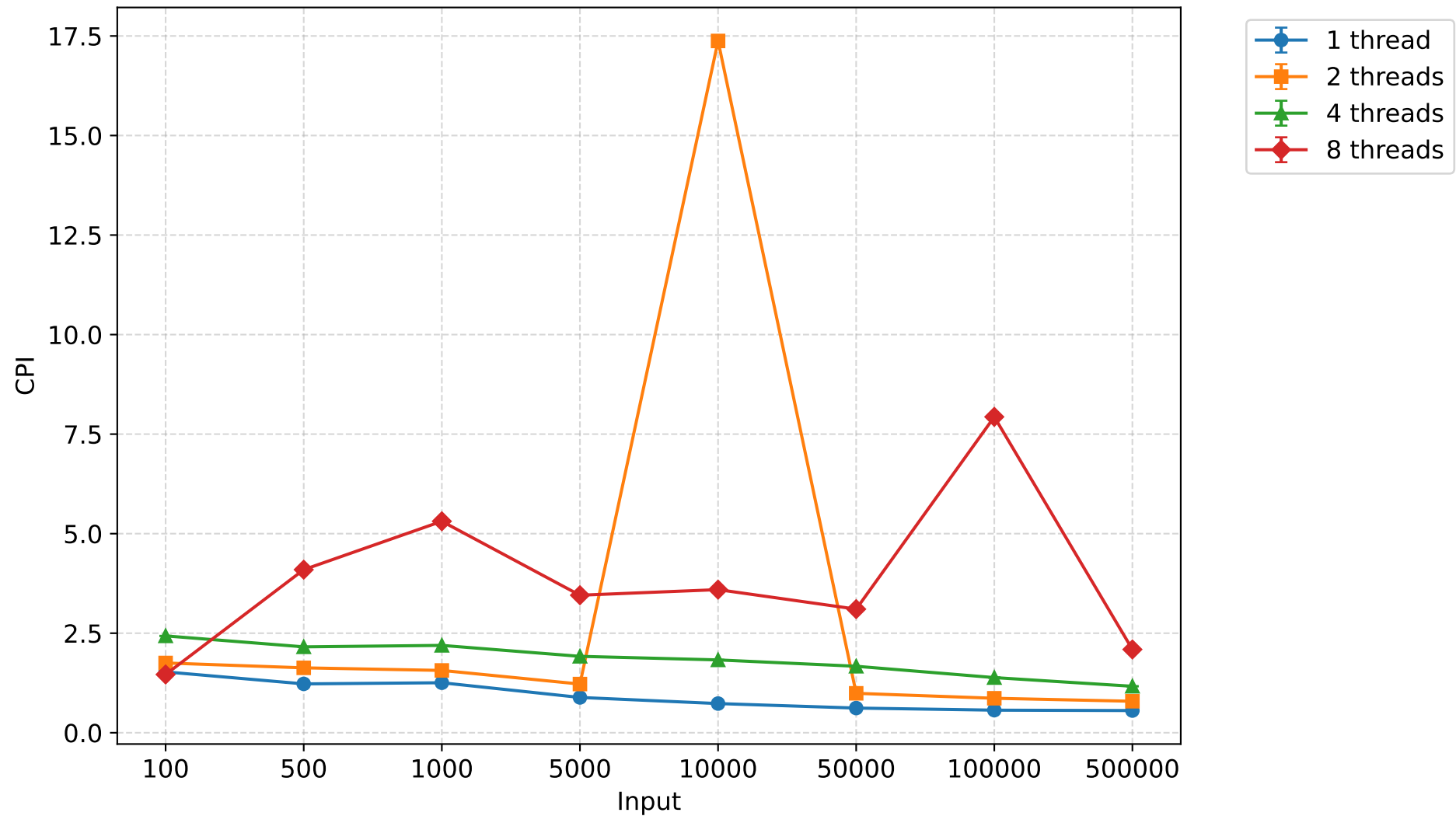
CPI - combort (mean \pm 95% CI)
