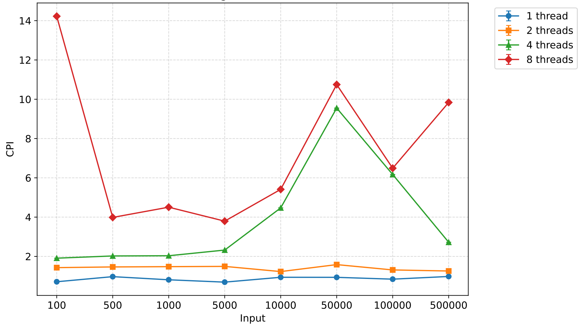
CPI - counting sort (mean \pm 95% CI)
