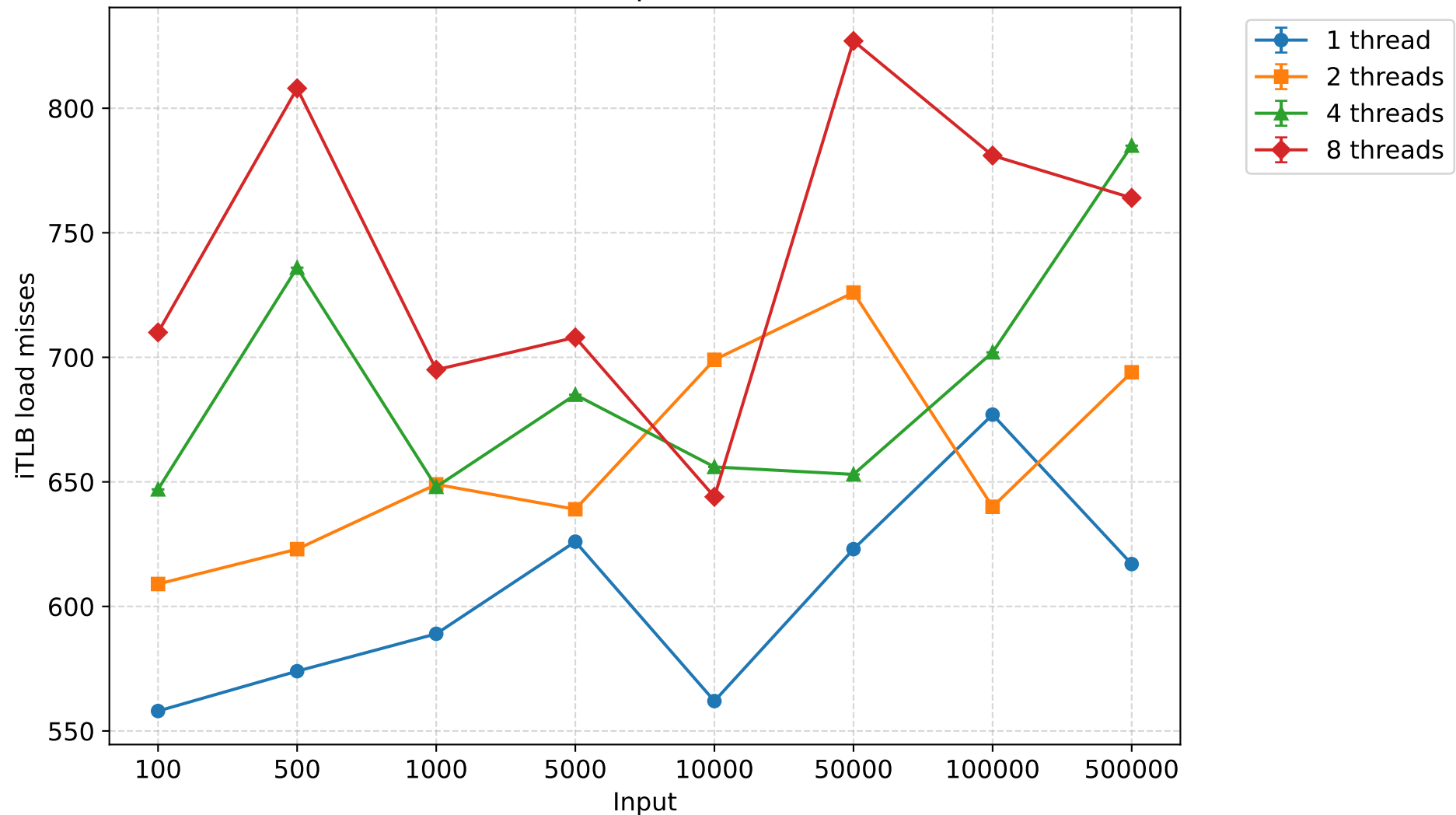
iTLB load misses - heapsort (mean \pm 95% CI)
