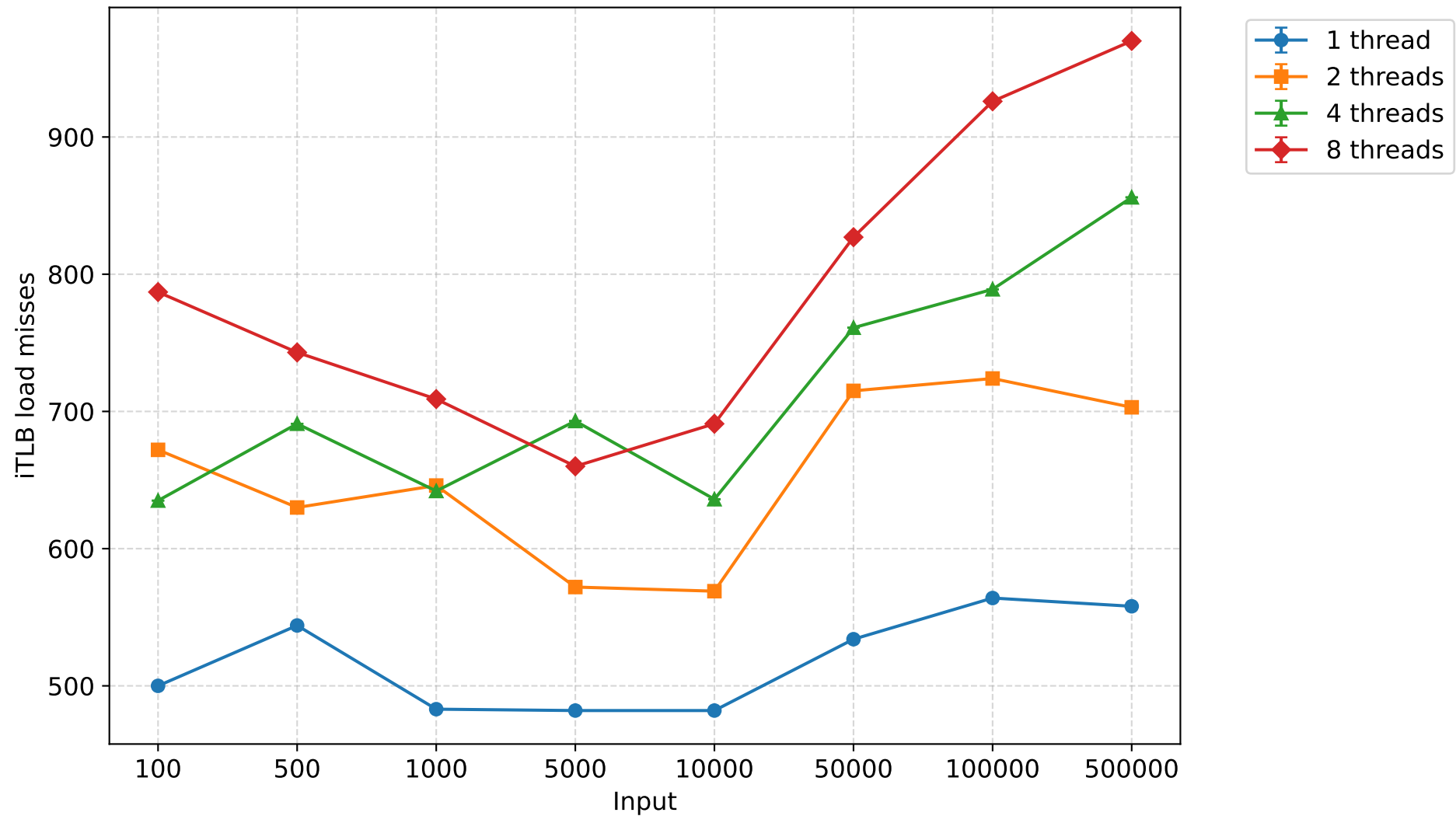
iTLB load misses - insertsort (mean \pm 95% CI)
