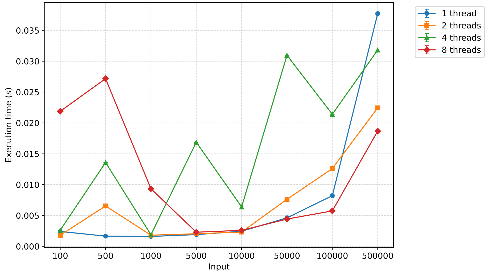
Execution time (s) - insertionsort (mean \pm 95% CI)
