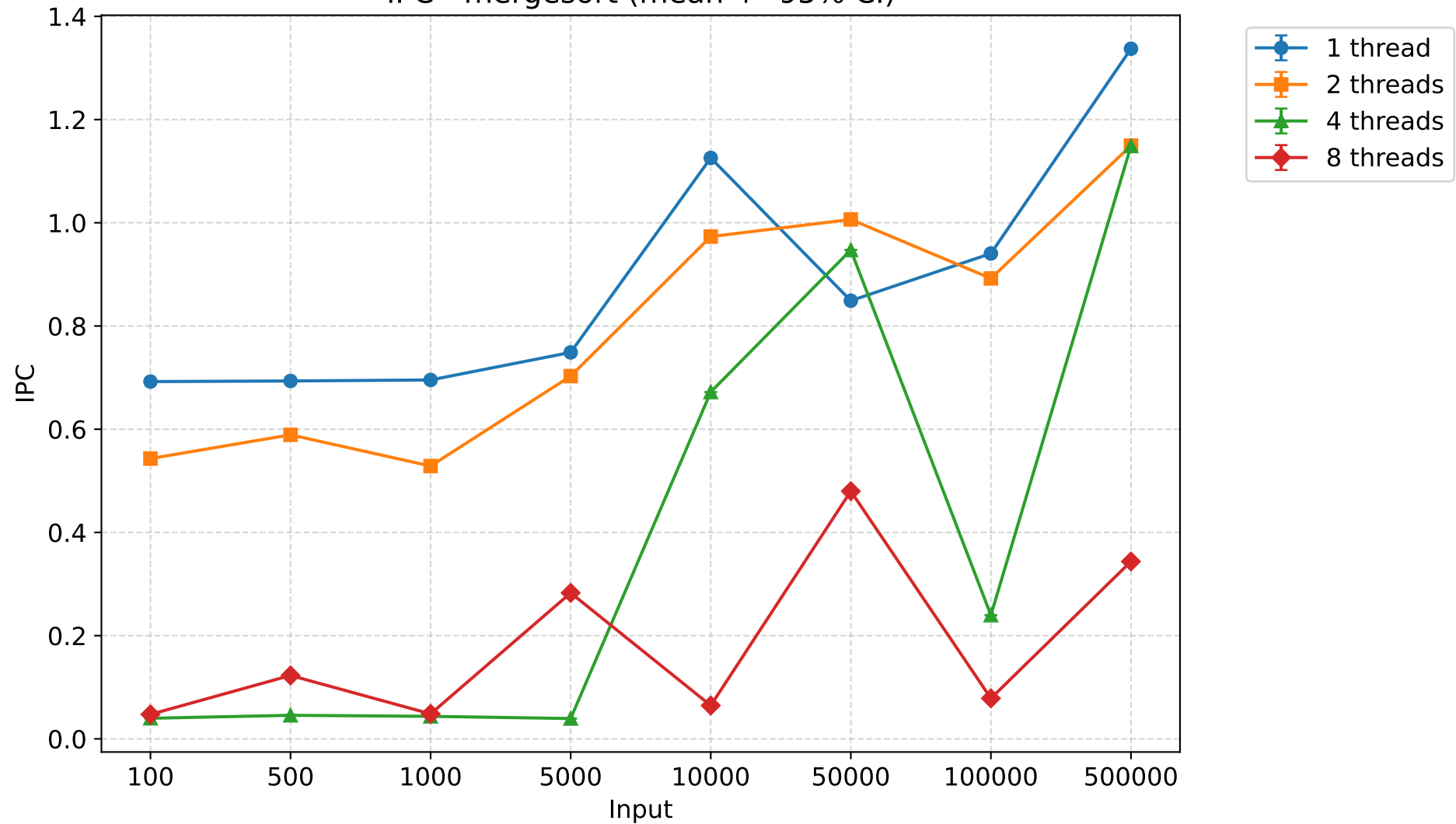
IPC - mergesort (mean \pm 95% CI)
