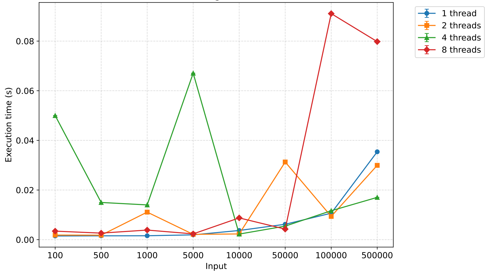
Execution time (s) - mergesort (mean \pm 95% CI)
