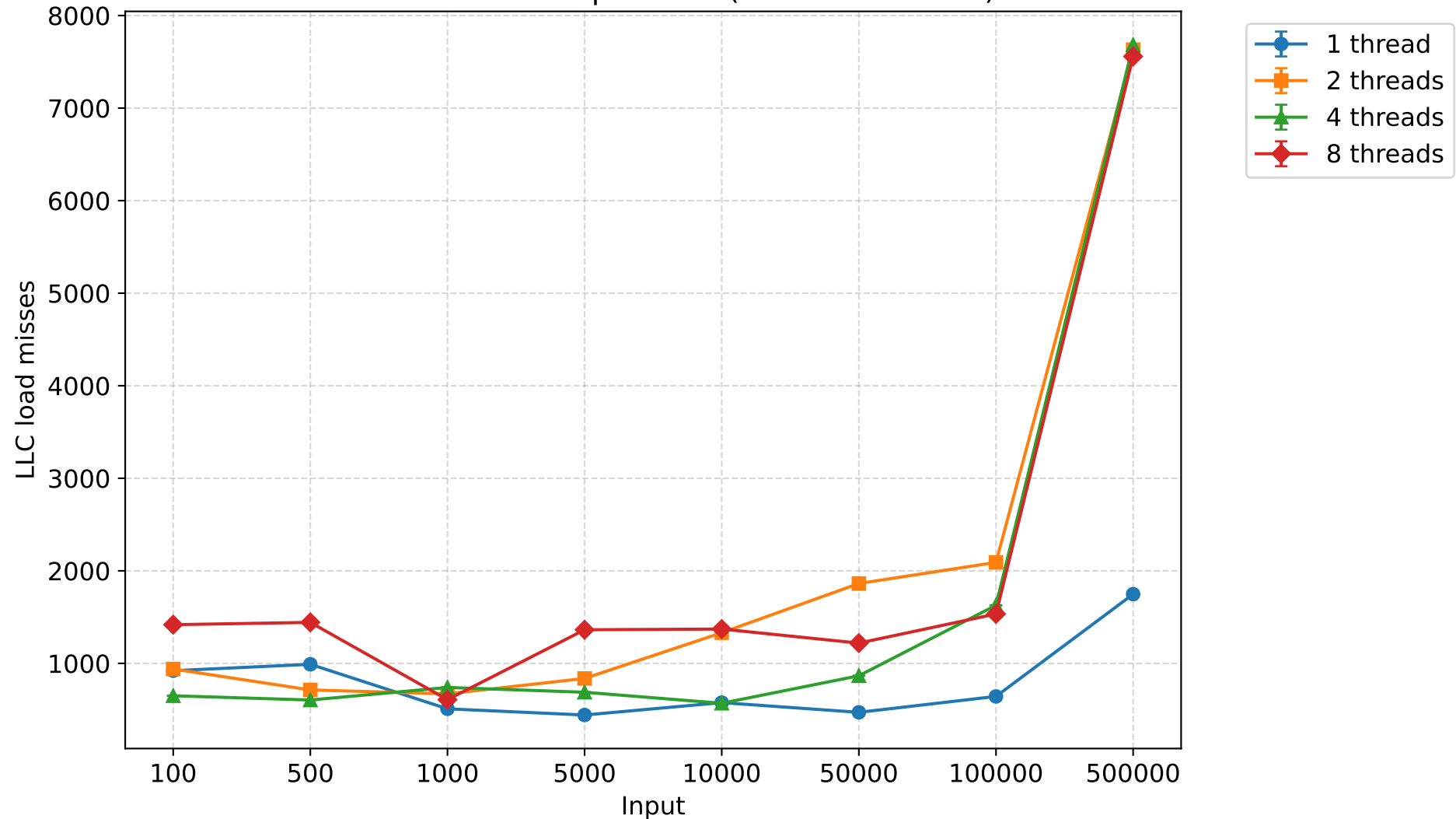
LLC load misses - quicksort (mean \pm 95% CI)
