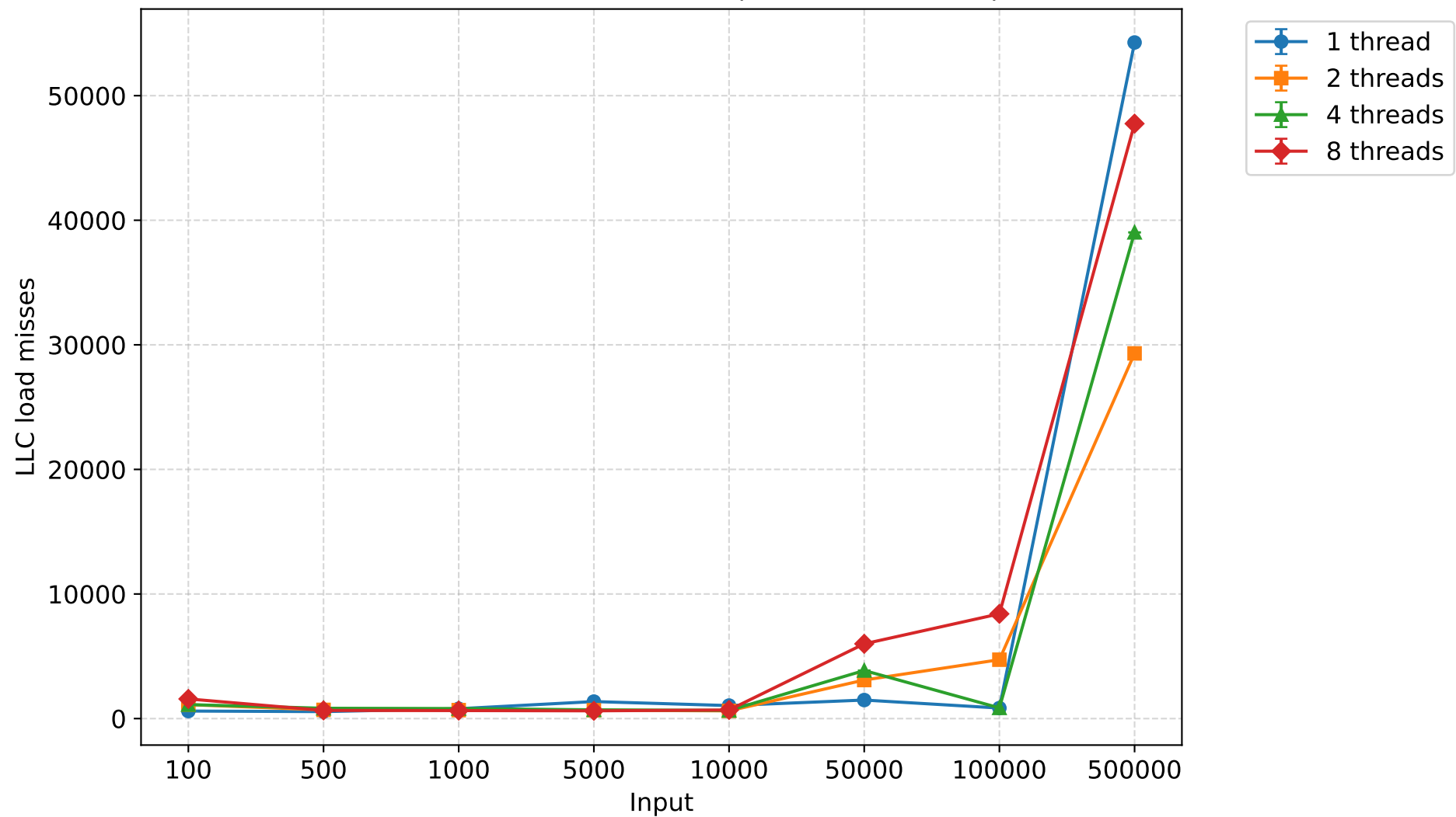
LLC load misses - radixsort (mean \pm 95% CI)
