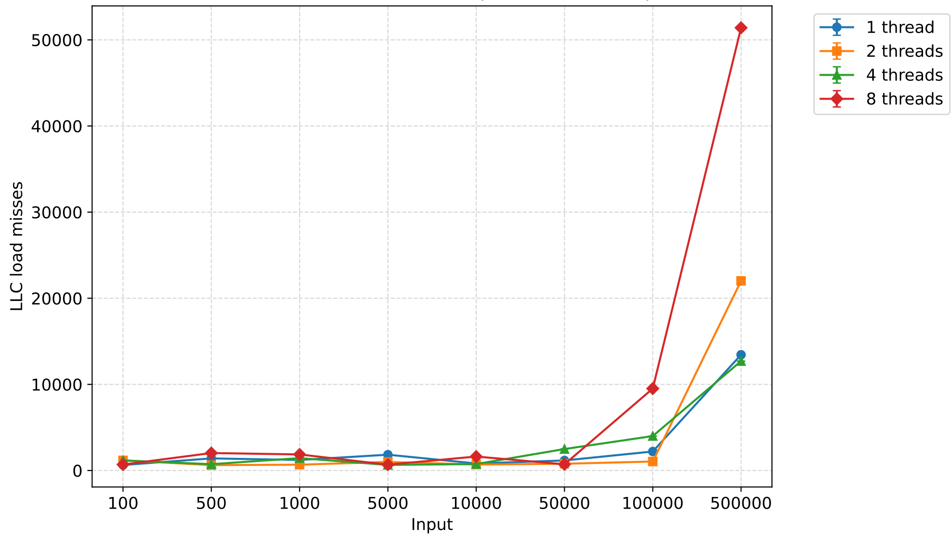
LLC load misses - shellsort (mean \pm 95% CI)
