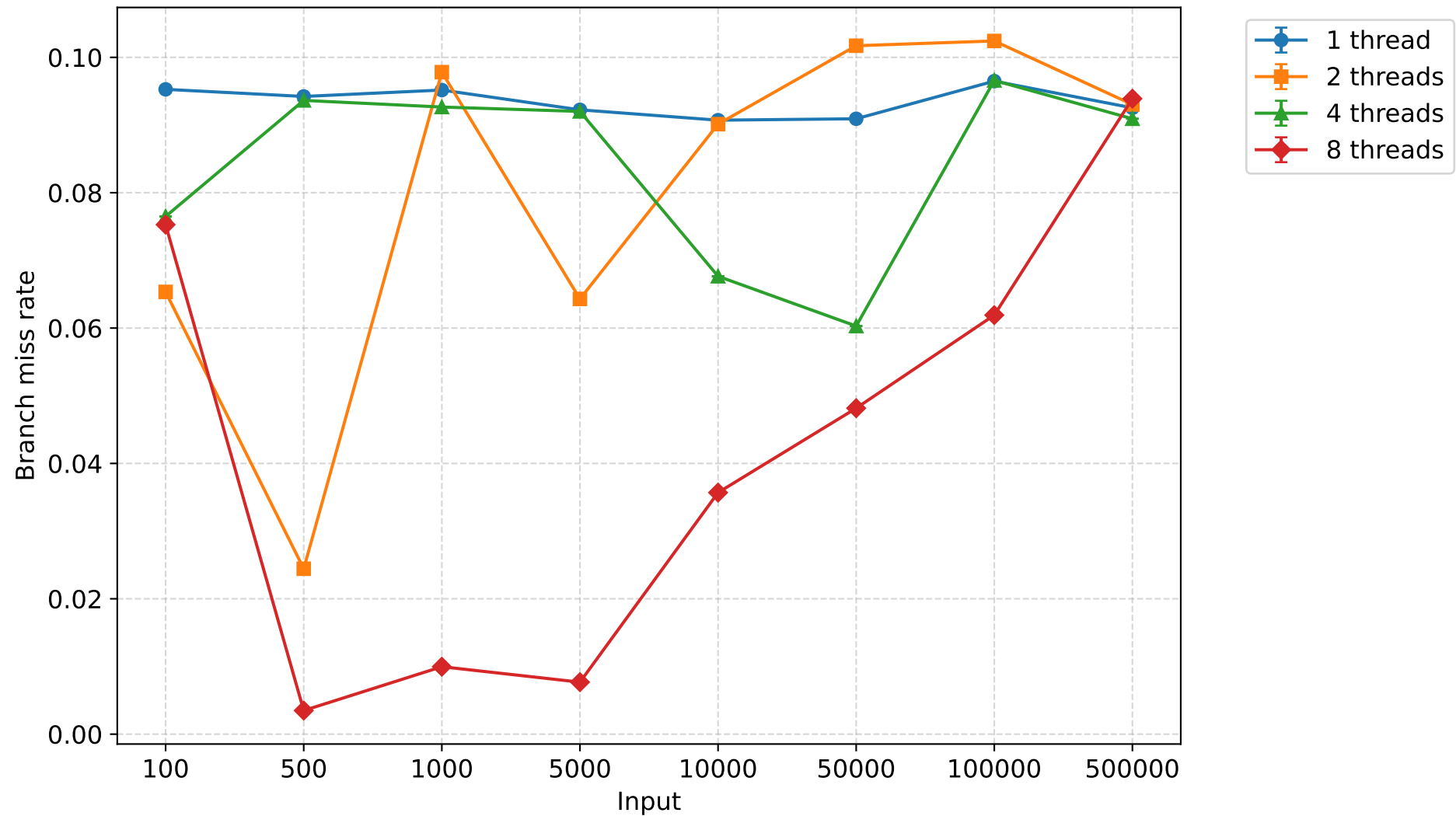
Branch miss rate - smoothsort (mean \pm 95% CI)
