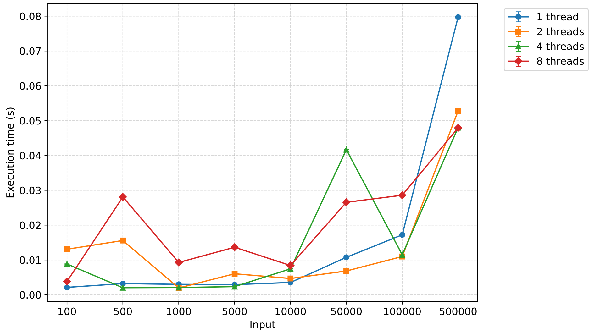
Execution time (s) - smoothsort (mean \pm 95% CI)
