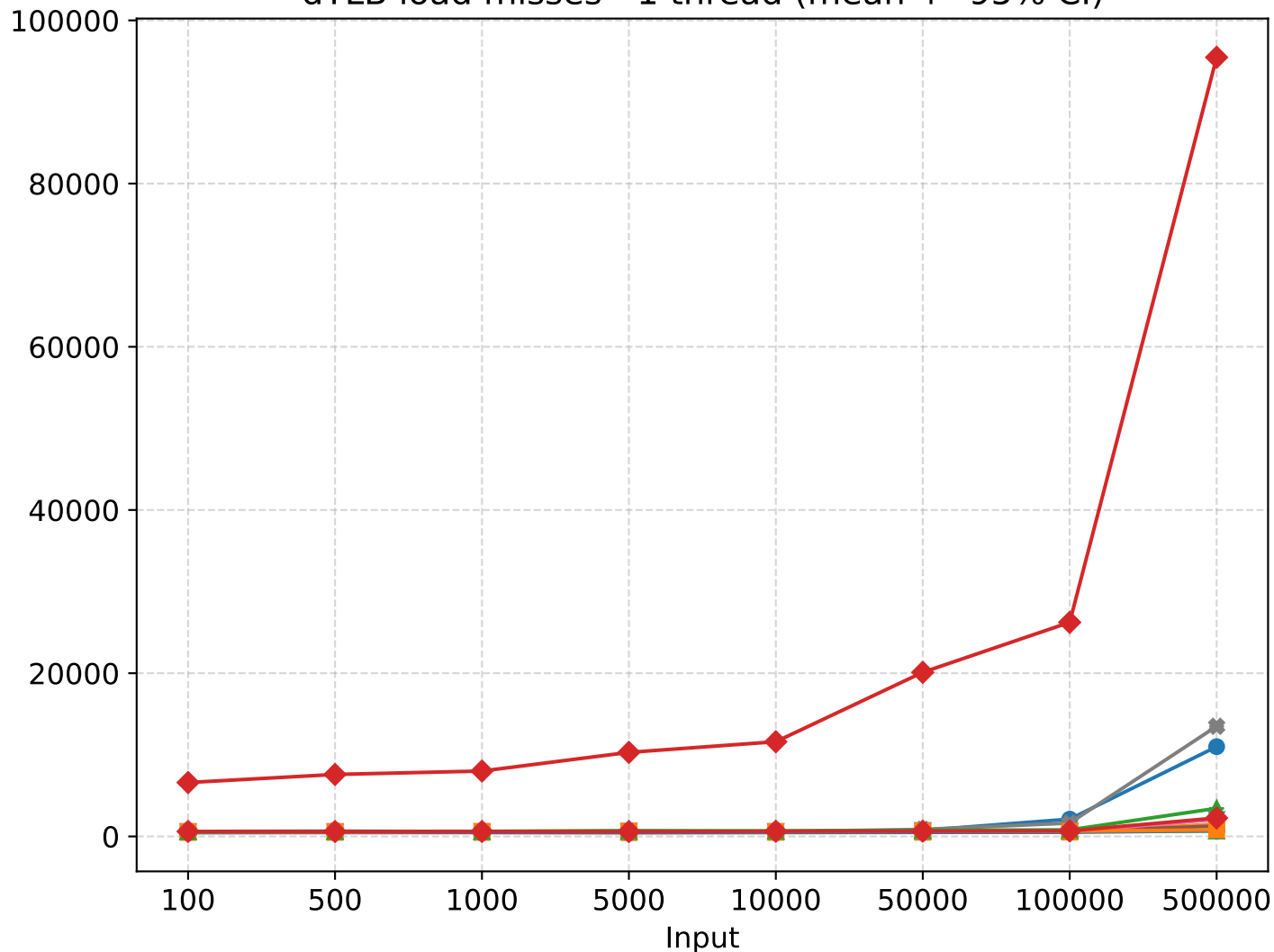
dTLB load misses - 1 thread (mean \pm 95% CI)
