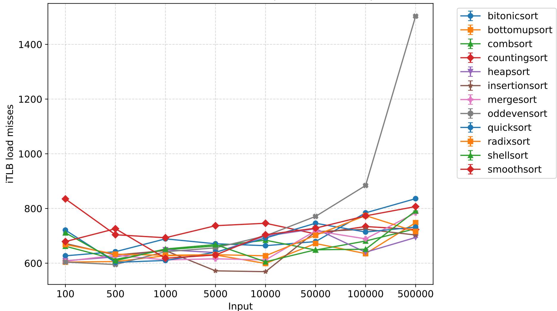
iTLB load misses - 2 threads (mean \pm 95% CI)
